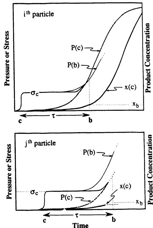
FIGURE 8. PRESSURE, STRESS, AND PRODUCT CONCENTRATION PROFILES FOR THE TWO PARTICLES.
