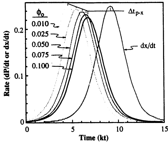
FIGURE 5. PRESSURE RATE AS A FUNCTION OF INITIAL POROSITY.
