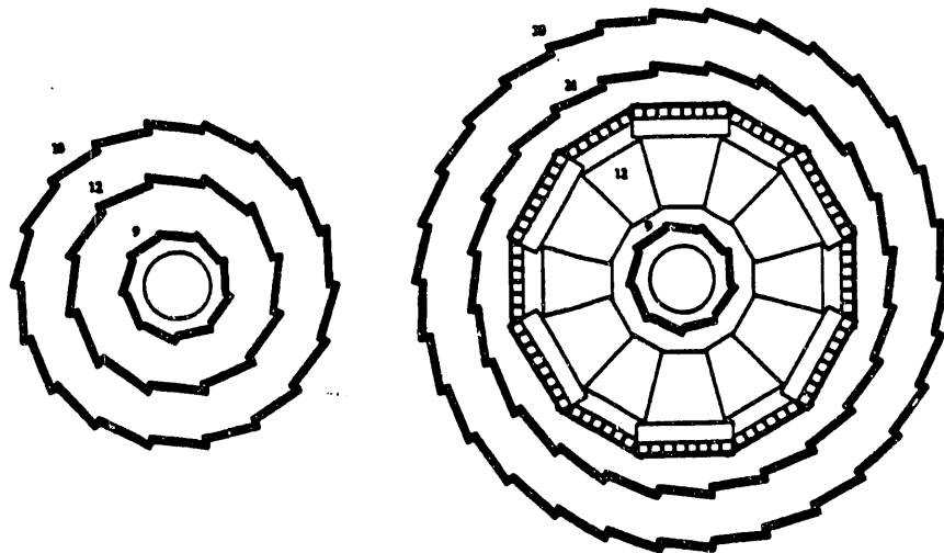
Figure 3: Cross-sections through the Step 1 barrels and Step 2 E-disk and barrels.
