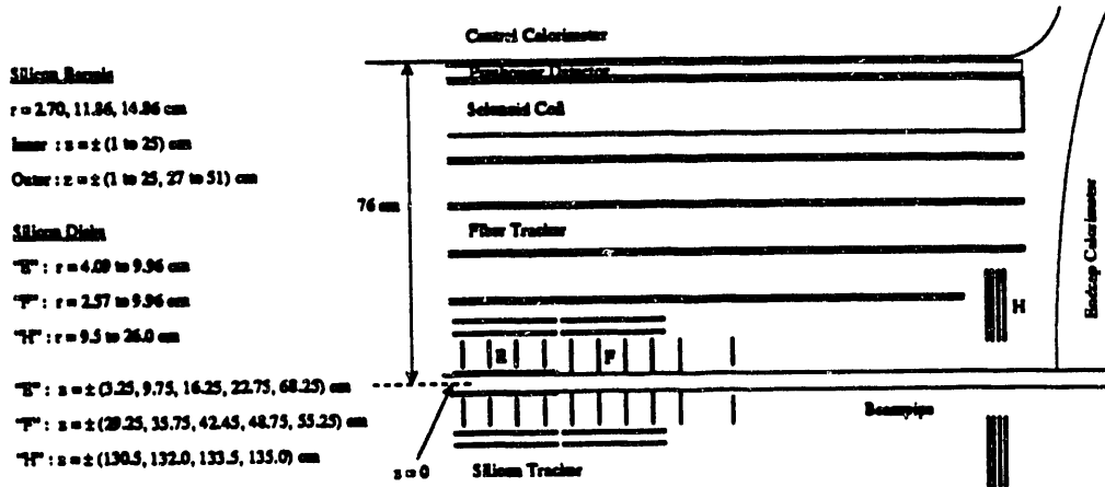
Figure 1: One quarter of the DO Step 1 upgrade tracking system.
