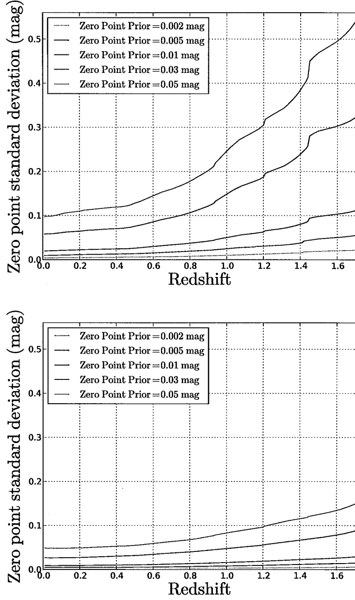
Fig. 1.— Zero-point covariance matrices standard deviations \sigma_a derived from MC, for different values of the zero-point priors, as a function of redshift. Upper panel: fitting for B_V \equiv A_V/R_V . Lower panel: fixing R_V = 3.1 . The two panels have the same scale to show how fitting for B_V significantly increases \sigma_a .
