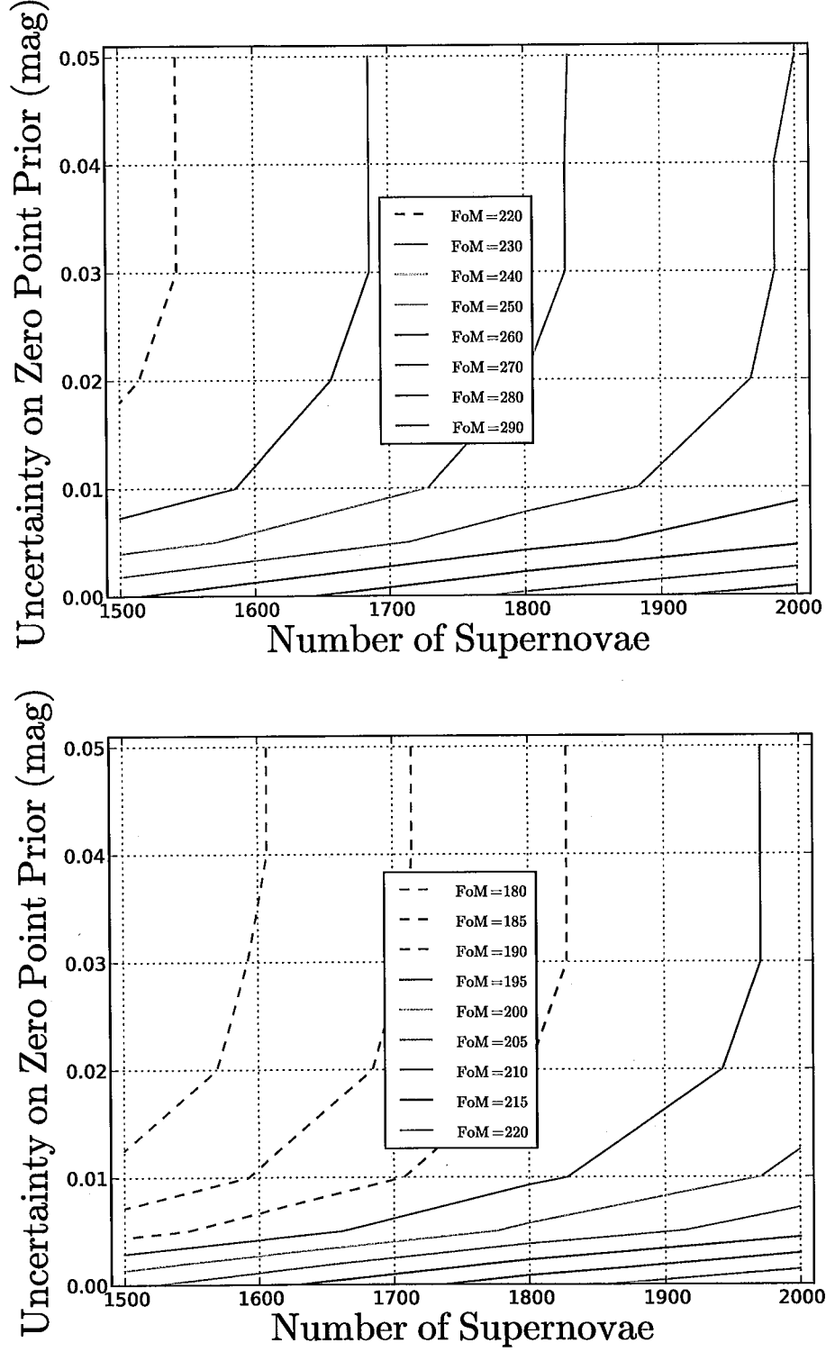
Fig. 7.— Contours of constant FoM for different uncertainties on the zero-point prior \sigma_Z and maximum number of supernovae N_{\text{SN}} . We assume z_{\text{max}} = 1.5 and \delta_c = 0.01 mag. Upper panel: the LH systematic is not included. Lower panel: the LH systematic is included.
