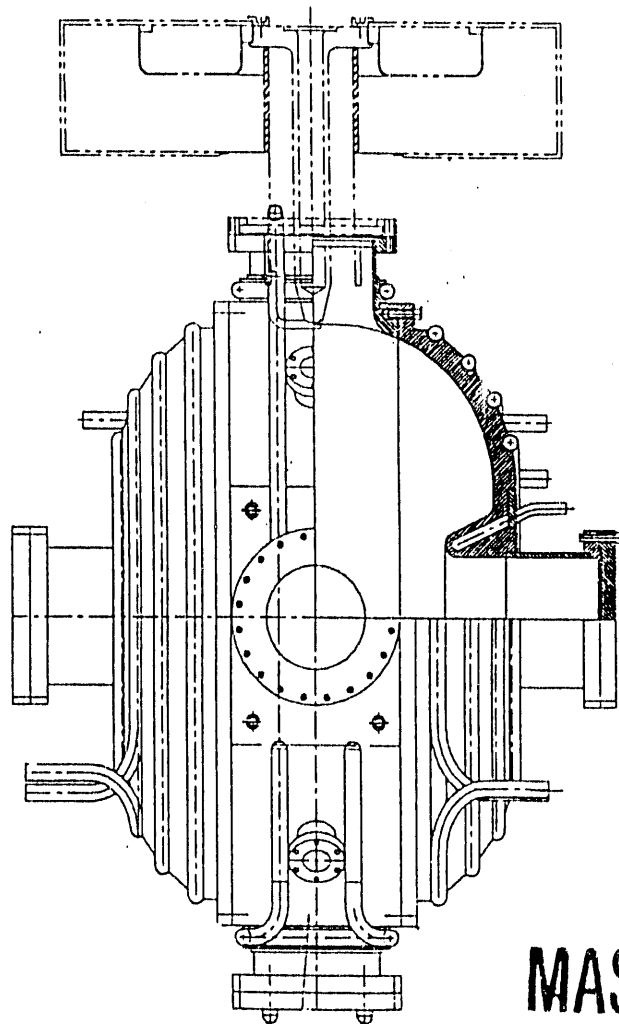
Figure 1. Prototype Storage Ring Cavity
