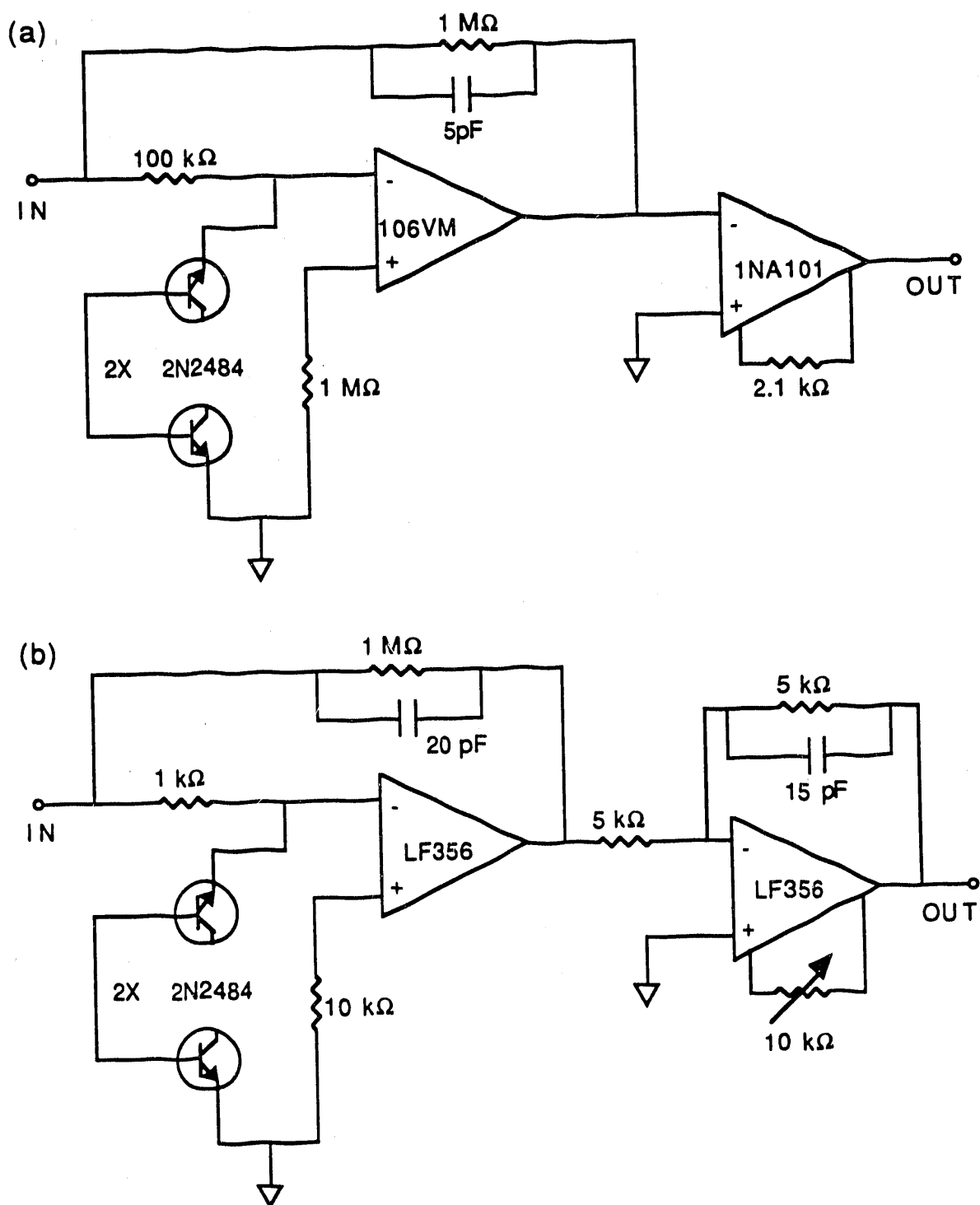
Figure 2-5 Schematics of the two pre-amplifiers used for this work. (a) Original pre-amplifier. (b) Improved pre-amplifier with higher gain.
