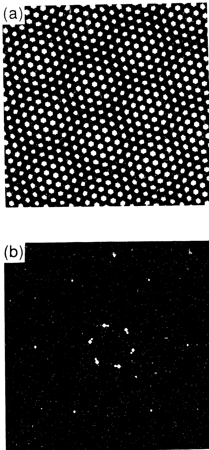
Figure 6-3 (a)Real space computer generated model of a discommensurate CDW with the parameters given by Nakanishi and Shiba in their proposed model for the configuration of the CDW in the NC phase of 1T-TaS 2 . (b) Fourier transform of (a). (XBB-910-8778A)
