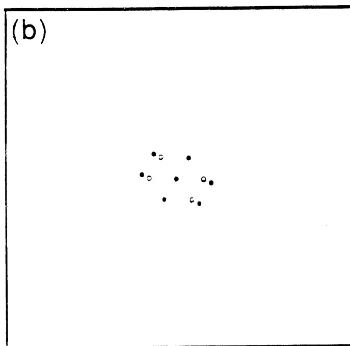
Figure 8-9 (a) Fourier transform of Fig. 8-8 showing the atomic lattice peaks. The two weak peaks nearest the center of the transform are due to 60 Hz noise on the feedback signal. (XBB-915-3889) (b) Schematic showing the calculated positions of the atomic lattice peaks (solid circles) and the CDW peaks (open circles).
