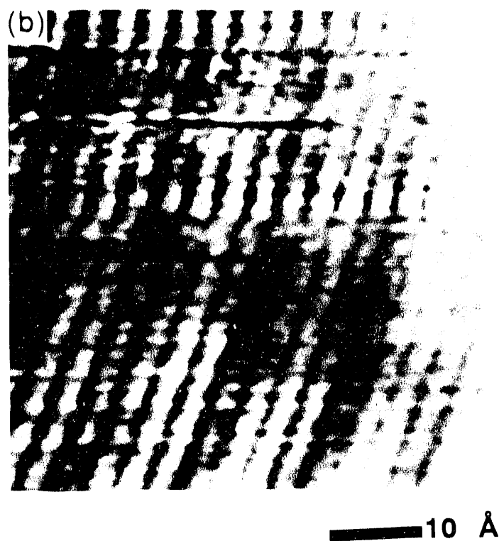
Figure 9-1. STM images of o-TaS 3 taken at 295K. Both the lattice and the CDW superstructure are clearly imaged in one dimension in both images. (XBB-910-8950A)
