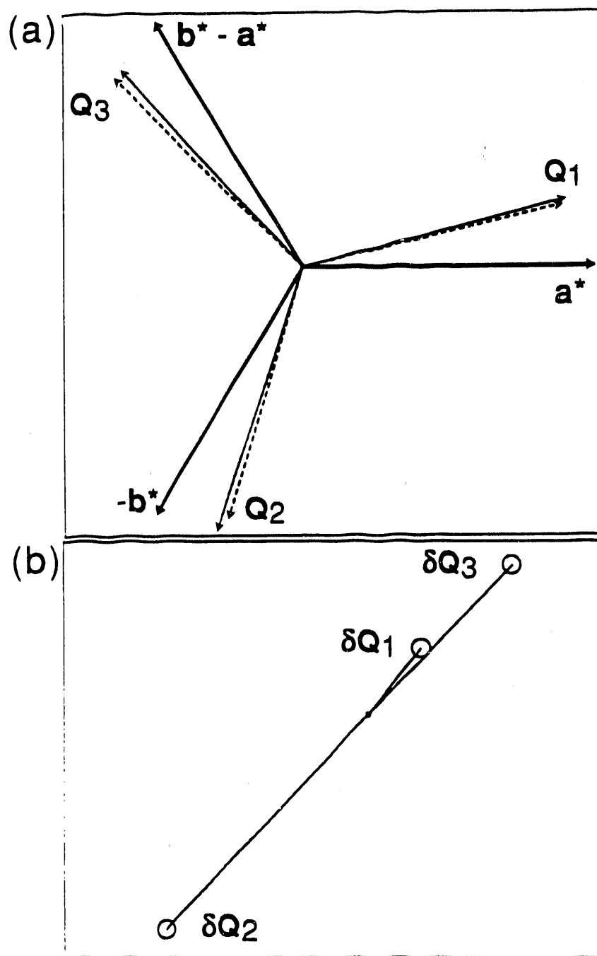
Figure 7-6 X-ray diffraction study results (a) plot of the fundamental CDW wavevectors relative to the commensurate wavevectors, (b) plot of the deviations of the fundamental CDW wavevectors from the commensurate wavevectors (Drawings courtesy of B. Burk.)
