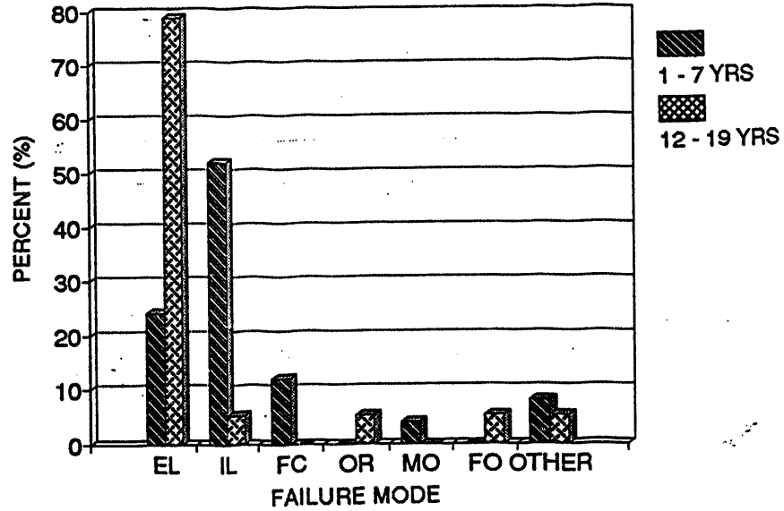
Figure 7. Failure modes for water valves
