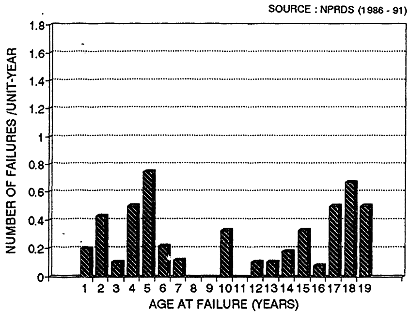
Figure 5. Normalized water valve failure frequency as a function of age at failure
