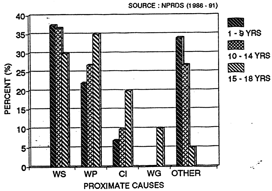
Figure 9. Proximate causes for steam valve failures
