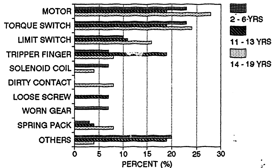
Figure 13. Proximate causes for valve operator failures
