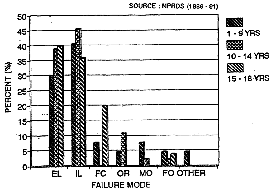
Figure 6. Failure modes for steam valves
