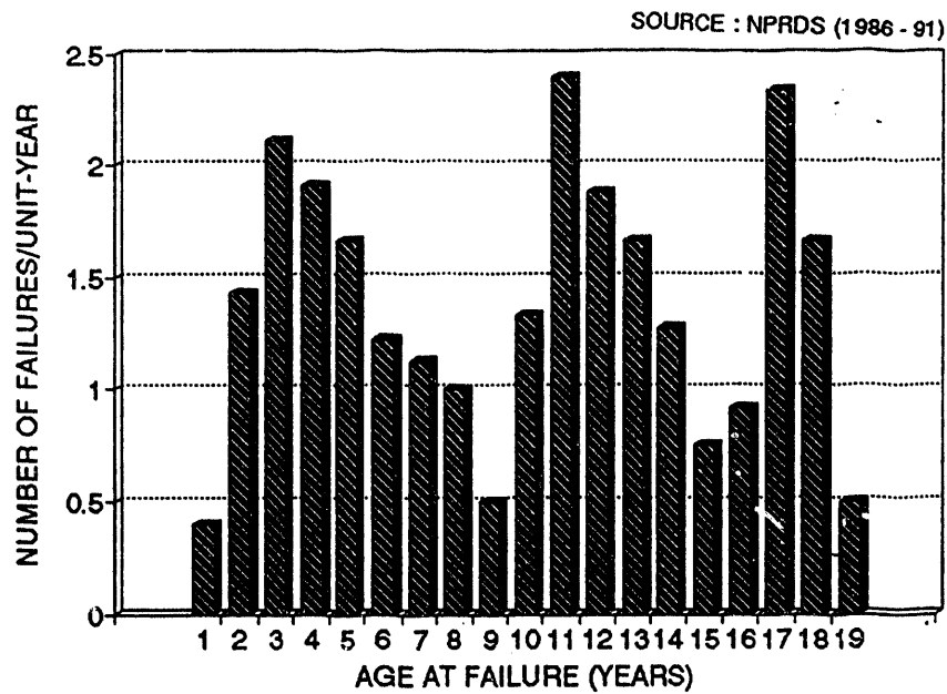
Figure 3. Normalized valve failure frequency as a function of age at failure
