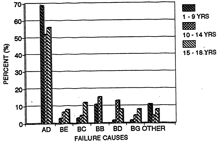
Figure 8. Failure causes for steam valves
