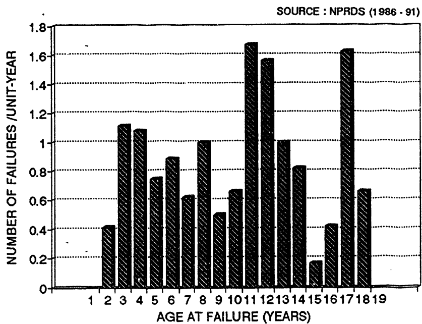
Figure 4. Normalized steam valve failure frequency as a function of age at failure
