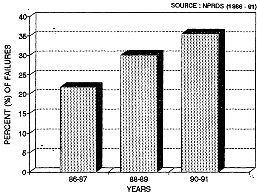
Figure 1. Fraction of RCIC component failures that caused loss of system function or degraded system operation
