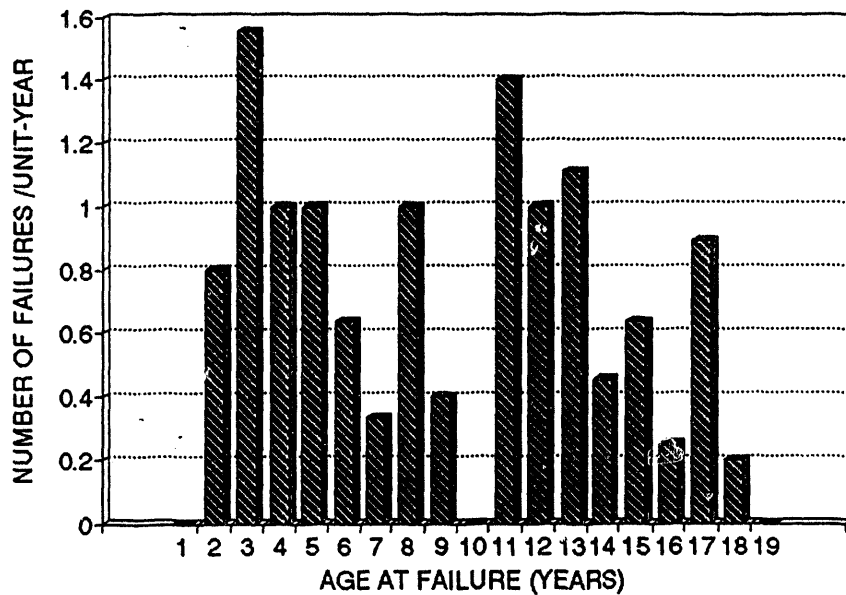
Figure 11. Normalized failure frequency for valve operators as a function of age at failure
