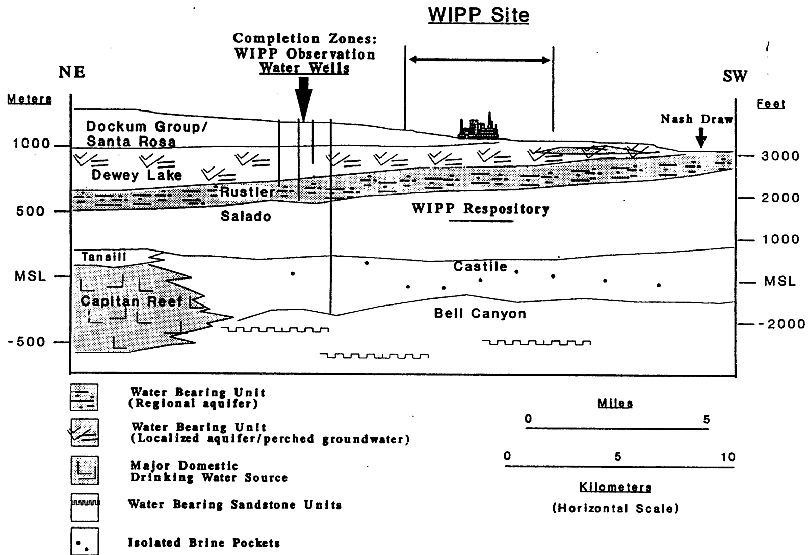
Schematic geologic cross-section illustrating key hydrogeologic units. (Modified after Kenney, 1991)
