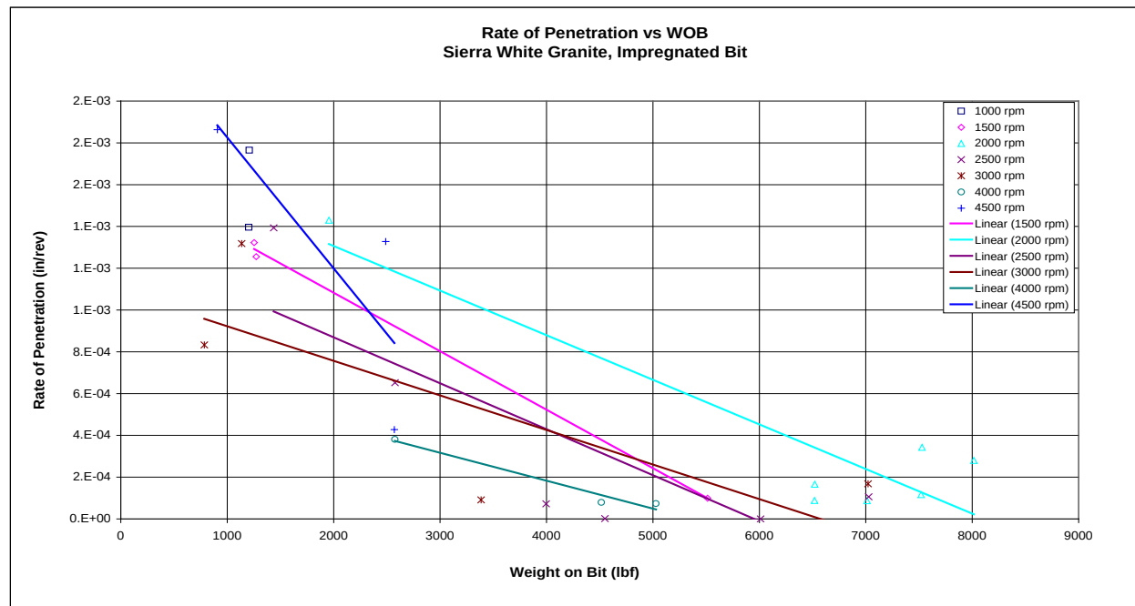
Figure 23. Rate of penetration is plotted as a function of weight on bit in Sierra White Granite with an impregnated drill bit. The trend lines plot data with similar rotary speeds.
