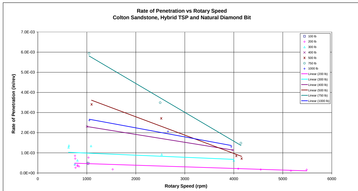
Figure 30. Rate of penetration is plotted as a function of rotary speed in Colton Sandstone with a hybrid natural diamond and TSP drill bit.
