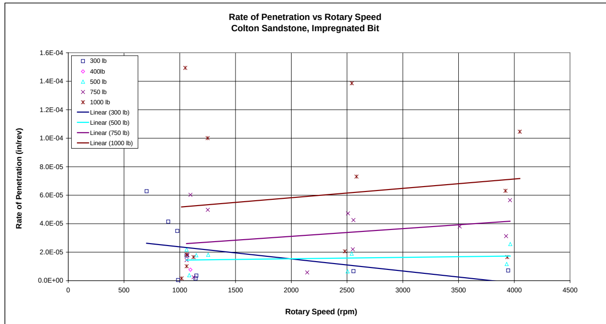
Figure 29. Rate of penetration is plotted as a function of rotary speed in Colton Sandstone with an impregnated drill bit.
