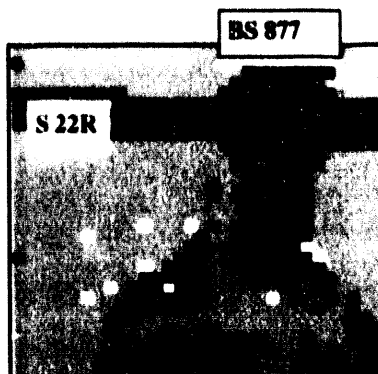
Failure Analysis ultrasonic array 8 x 8 inch C-scan image at BS 877. Area of corrosion is shown in light blue surrounded by green.
