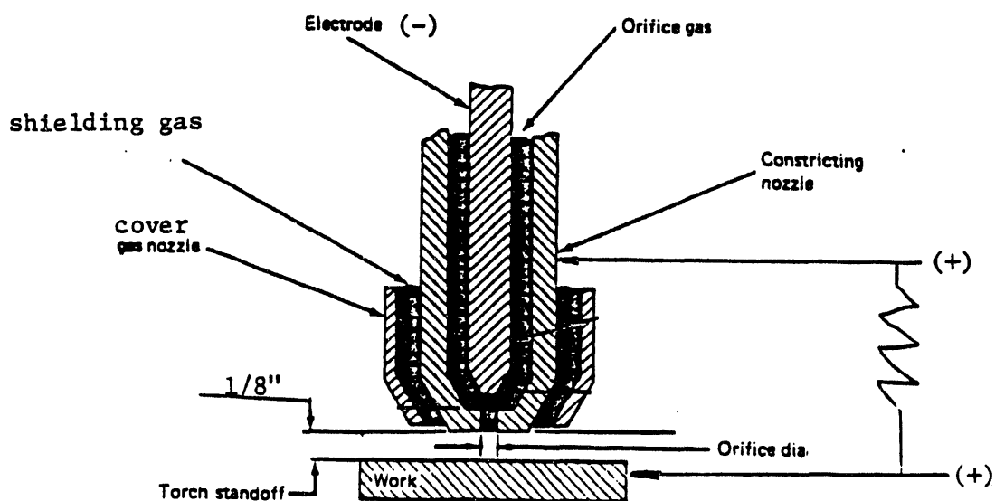
Figure 3 - Configuration of the plasma arc torch head.
