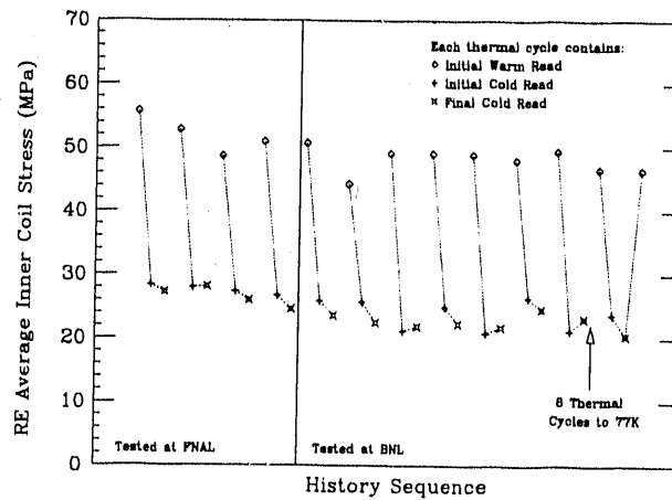
Figure 2. Inner coil stress history of return end gauge pack. Each thermal cycle contains an initial warm, cold, and final cold read.
