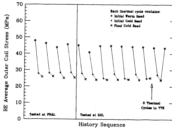
Figure 3. Outer coil stress history of return end gauge pack. Each thermal cycle contains an initial warm, cold, and final cold read.
