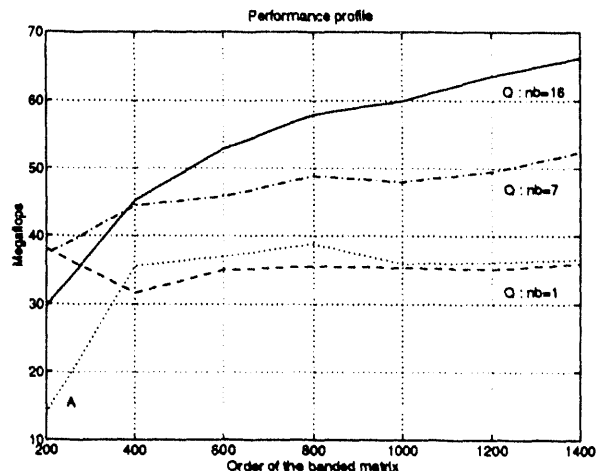
Figure 4: Performance of the Reduction and of the Update on a Single Node of the IBM SP1
