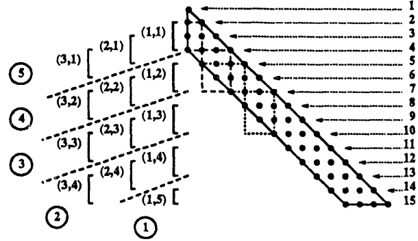
Figure 2: Illustration of the Tridiagonalization Algorithm
