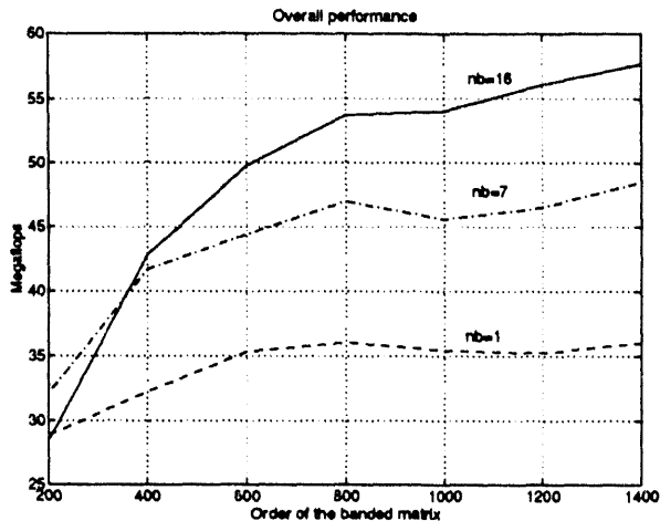
Figure 3: Tridiagonalization Performance (including Accumulation of Q ) on a Single Node of the IBM SP1
