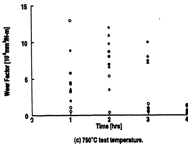
Figure 5.—Block wear variation with time at the different test temperatures.
