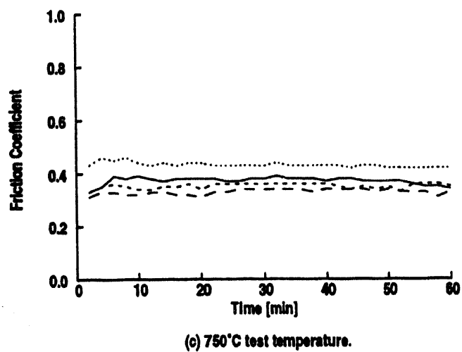
Figure 4.—Comparison of average friction coefficient versus time for all rub blocks at the different test temperatures.
