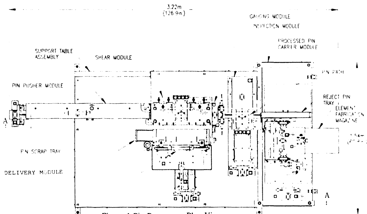
Figure 1 Pin Processor - Plan View
