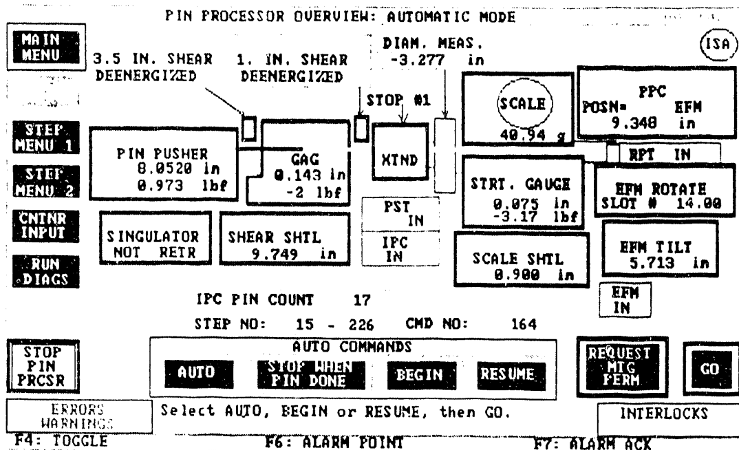
Figure 3 Pin Processor Operator Control Automatic Overview Screen
