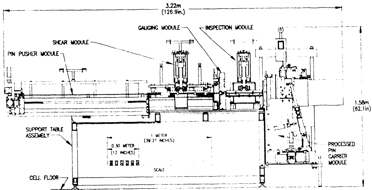
Figure 2 Pin Processor - Section Through Pin Path
