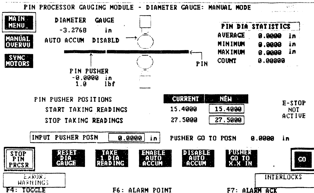
Figure 4 Pin Processor Operator Control Manual Control Screen
