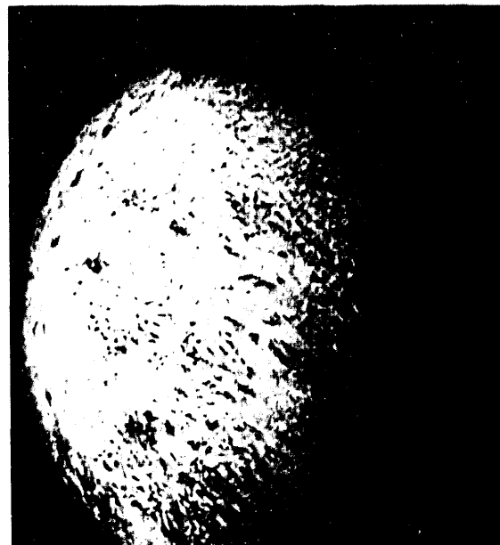
Neptune, currently the outermost planet in the solar system, and its largest satellite, Triton, were imaged close-up by NASA's Voyager 2 spacecraft in August 1989. Four times Earth's diameter but 30 times Earth's distance from the sun, Neptune is invisible to the naked eye. It was not even discovered until 1846 and appears little larger than the resolution limit of even the largest ground-based telescopes. Space missions such as Voyager involve large numbers of scientists, engineers, and mathematicians (NASA photographs)
