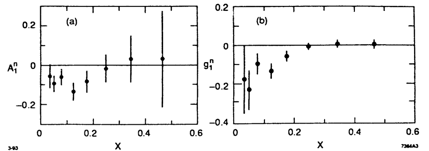
Fig. 2. (a) Neutron asymmetries A_1^n and (b) spin-structure function g_1^n , as a function of x .
