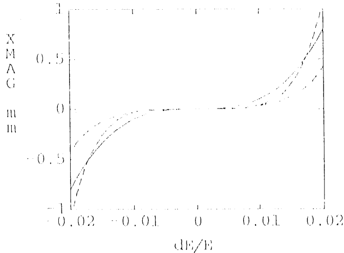
Figure 5: Third order dispersion.
