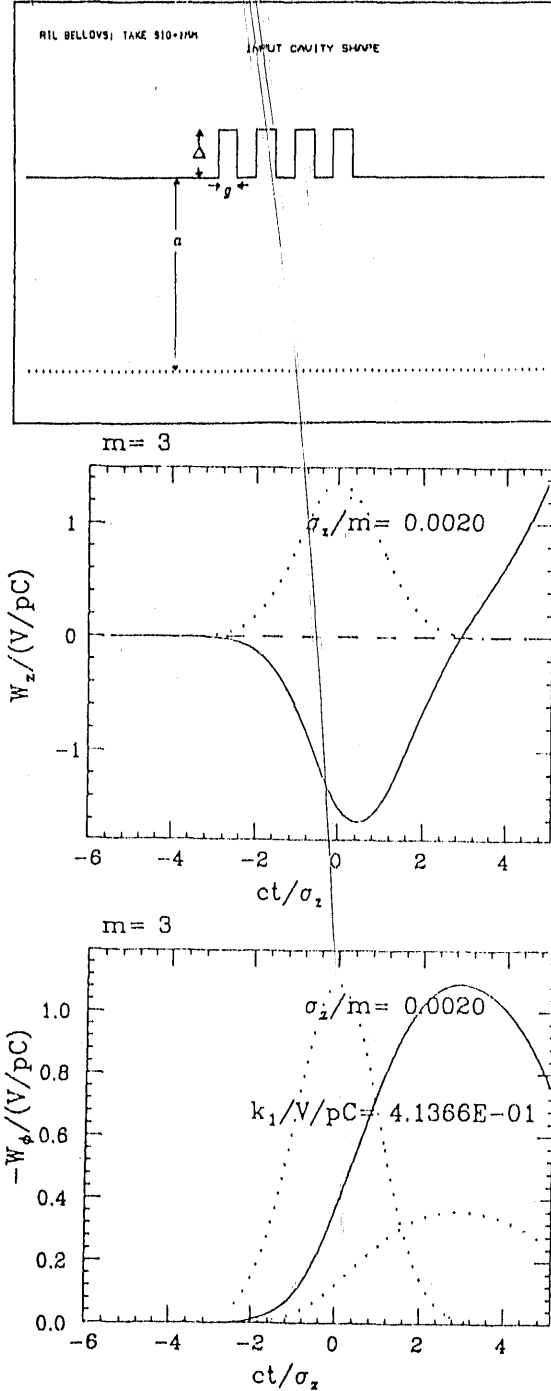
Figure 6: Wakefield calculation.
