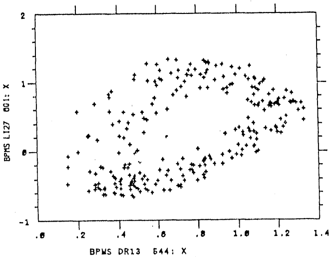
Figure 2: Donut Correlation.
