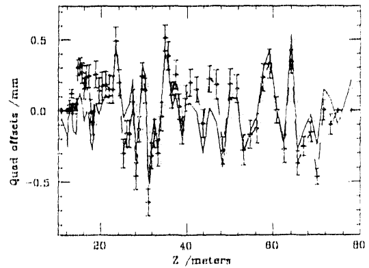
Fig 3. Quadrupole horizontal position offsets resulting from simulation conditions of Table 1. The true offsets (solid) and the fitted offsets (dashed) are shown and agree at frequencies > f_\beta .
