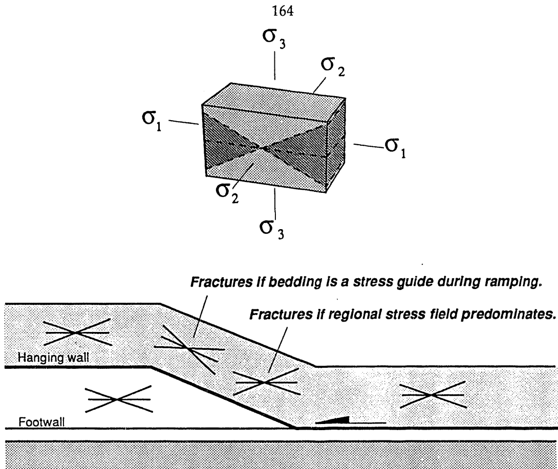
Fig. 5-37. Foreland fold-thrust belt structures, which can be used to infer the orientation of the regional stress field during their development. Shown are the orientations of the fractures that would form if the orientation of the regional stress field predominates across the thrust belt or if bedding acts as a local stress guide during ramping.
