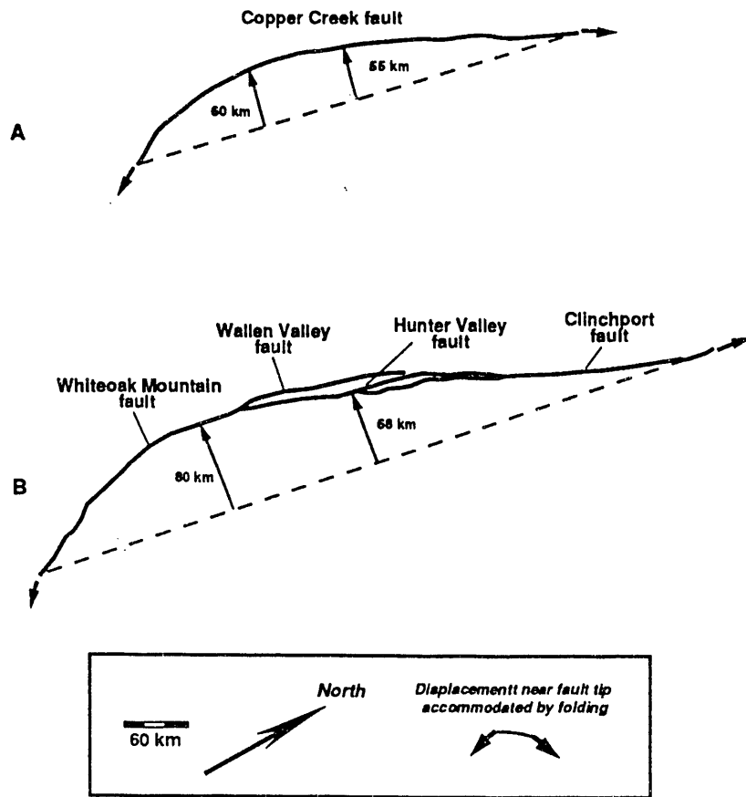
Fig. 5-6. Sketch of the map-view geometry of (A) the Copper Creek and (B) Whiteoak Mountain faults used to estimate displacement by the bow and arrow rule. Note that the length of the longest normal from the fault to the tip-line join results in greater displacement than if the middle of the tip-line join is chosen.
