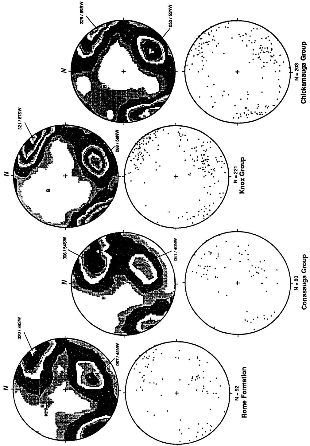
Fig. 5-26. Equal-area scatter and Kamb contour plots of poles to fracture planes for the Rome Formation, Conasauga Group, Knox Group, and Chickamauga Group in the Whiteoak Mountain thrust sheet. Contour interval is 1.0 sigma; B = mean pole to bedding.
