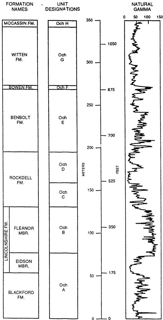
CHICKAMAUGA GROUP COMPOSITE GEOPHYSICAL LOG AND UNIT DESIGNATIONS
