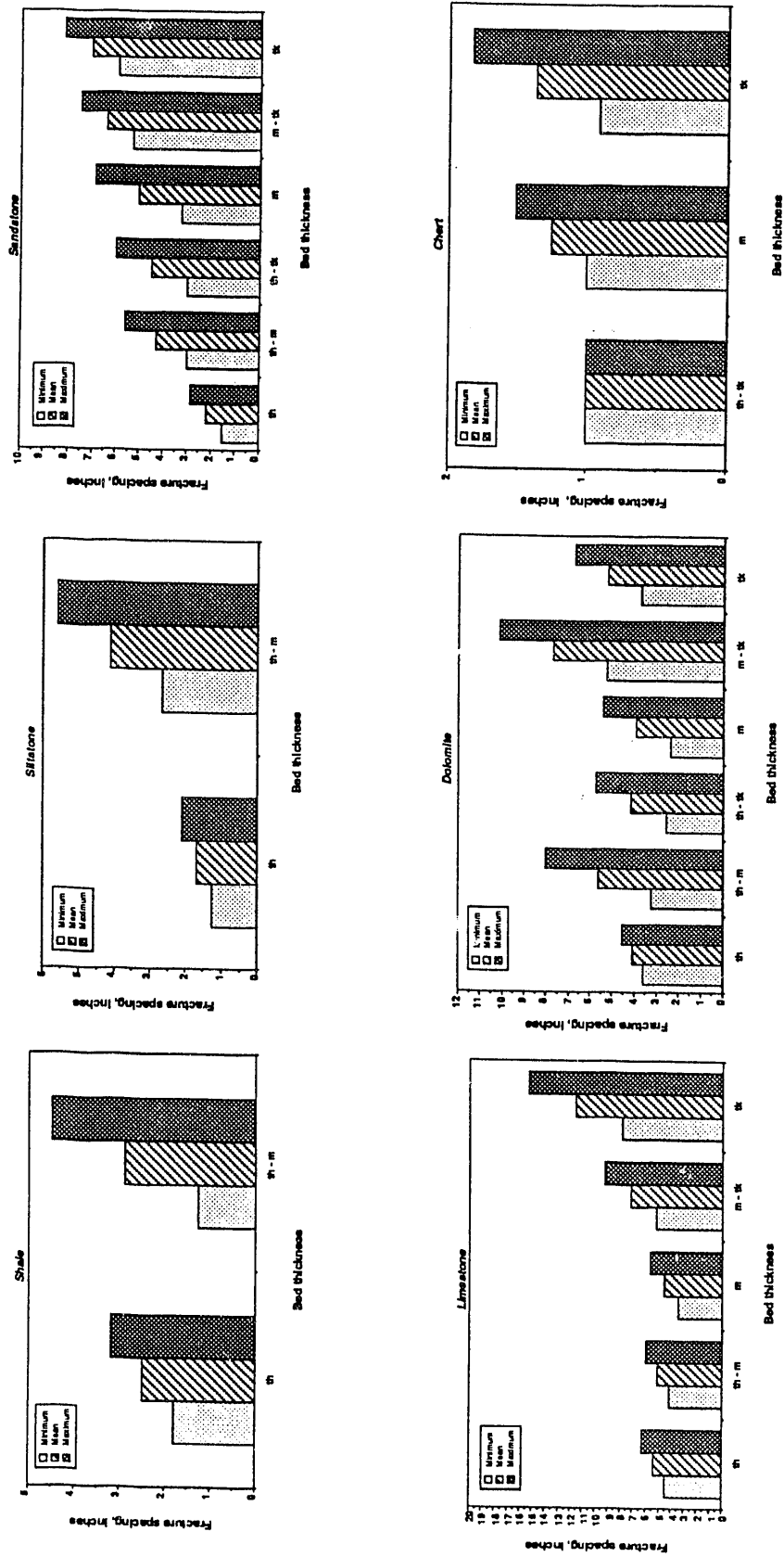
Fig. 5-45. Fracture spacing vs bed thickness for each lithology.
