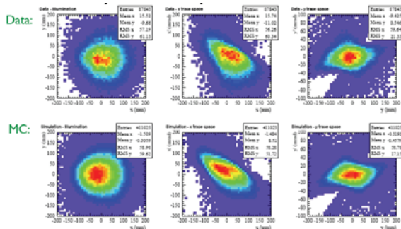
Figure 13: Plots of real-space (x,y) (left column), and phase-space (x,x') (middle column) and (y,y') (right column), distributions. The upper row shows measurements and the lower row shows the ability of Monte Carlo (MC) simulations to reproduce them.
