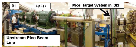
Figure 11: Upstream portion of MICE muon beam line. The ISIS ring is visible in the background.
