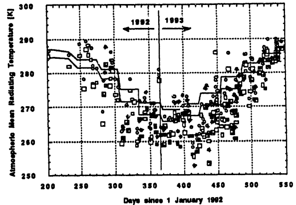
Figure 9. Mean radiating temperatures computed from soundings for 23.8 GHz (circles) and 31.4 GHz (squares) under cloudy sky (open symbols) and clear sky (symbols with '+'s) conditions. The monthly mean values used in the retrievals are indicated as solid lines. ( T_{mr, 23.8} > T_{mr, 31.4} )
