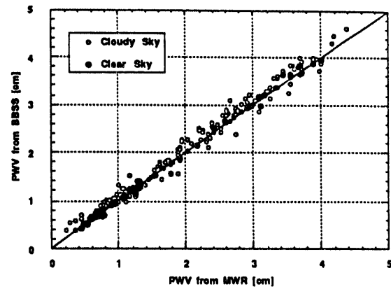
Figure 4. Scatter plot of PWV measured with the MWR against PWV derived from BBSS soundings for clear and cloudy sky conditions through June 1993.
