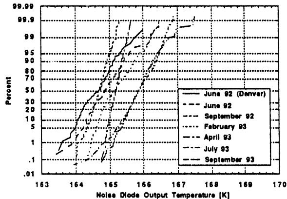
Figure 3. Noise diode output calibration history for the 31.4 GHz channel.
