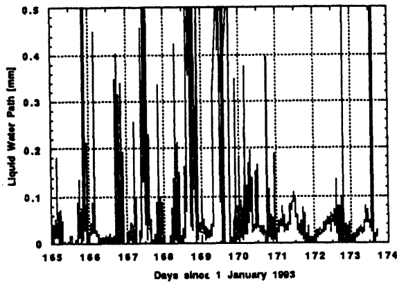
Figure 7. Time series of LWP for 15-23 June 1993.
