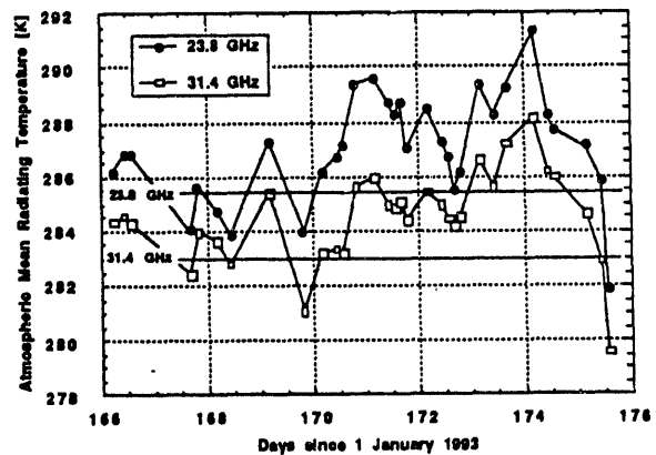
Figure 10. T_{mr} computed from soundings for 16-26 June 1993. Climatological average values for June are indicated as solid lines.
