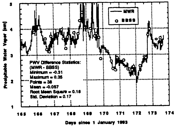
Figure 6. Time series of PWV for 15-23 June 1993.
