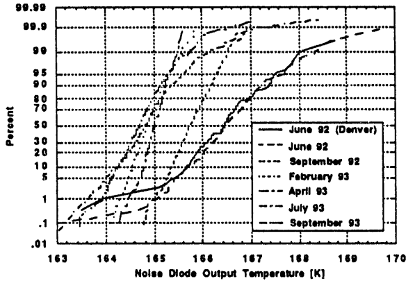
Figure 2. Noise diode output calibration history for the 23.8 GHz channel.
