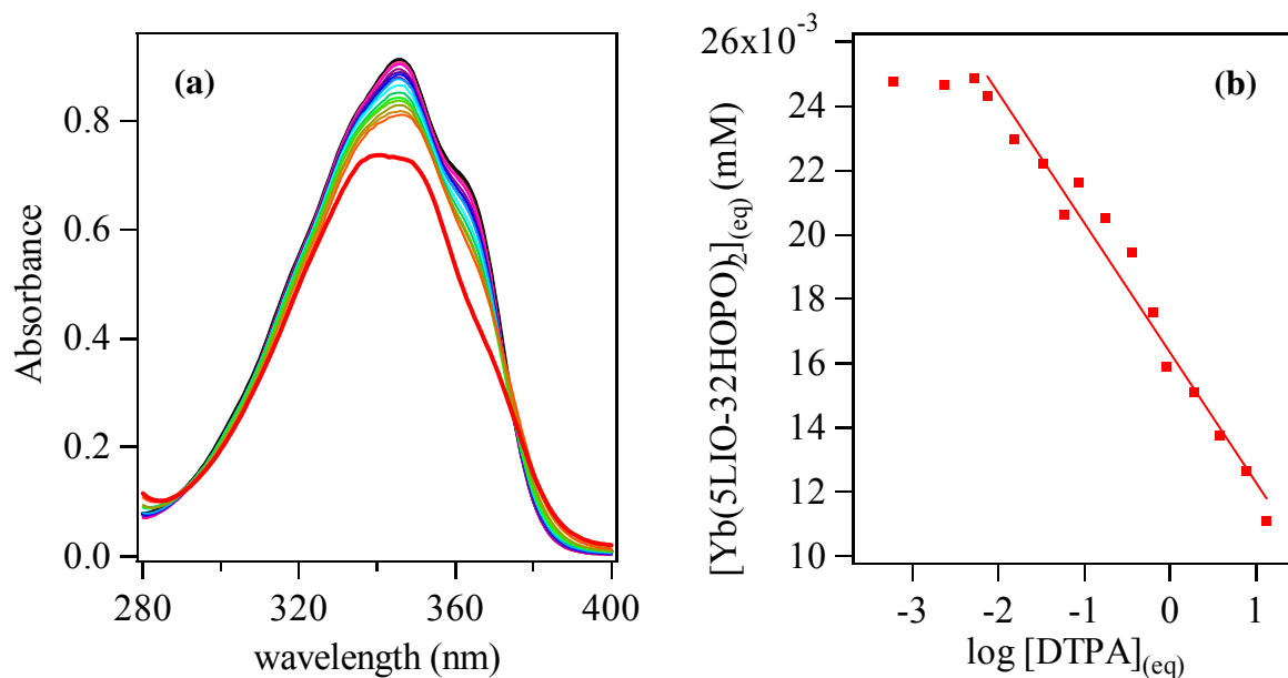
Figure 3. (a) Absorption spectra (left) for solutions of [\text{Yb}(\text{5LIO-Me-3,2-HOPO})_2]^- (26 μM in 0.1 M KCl; 0.01 M HEPES at pH 7.4; black line) and after addition of up to ca. 500 equivalents of DTPA (red). (b) Plot of equilibrium concentration (right) determined from absorption spectra versus equilibrium concentration of log DTPA ( \text{mM}^{-1} ) and corresponding fit used to evaluate equal speciation between 5LIO-Me-3,2-HOPO and DTPA ( i.e. 50 % [\text{Yb}(\text{DTPA})] at ca. 0.013 mM, which corresponds to a \text{pYb} = 18.8 (1) for the [\text{Yb}(\text{5LIO-Me-3,2-HOPO})_2] complex.
