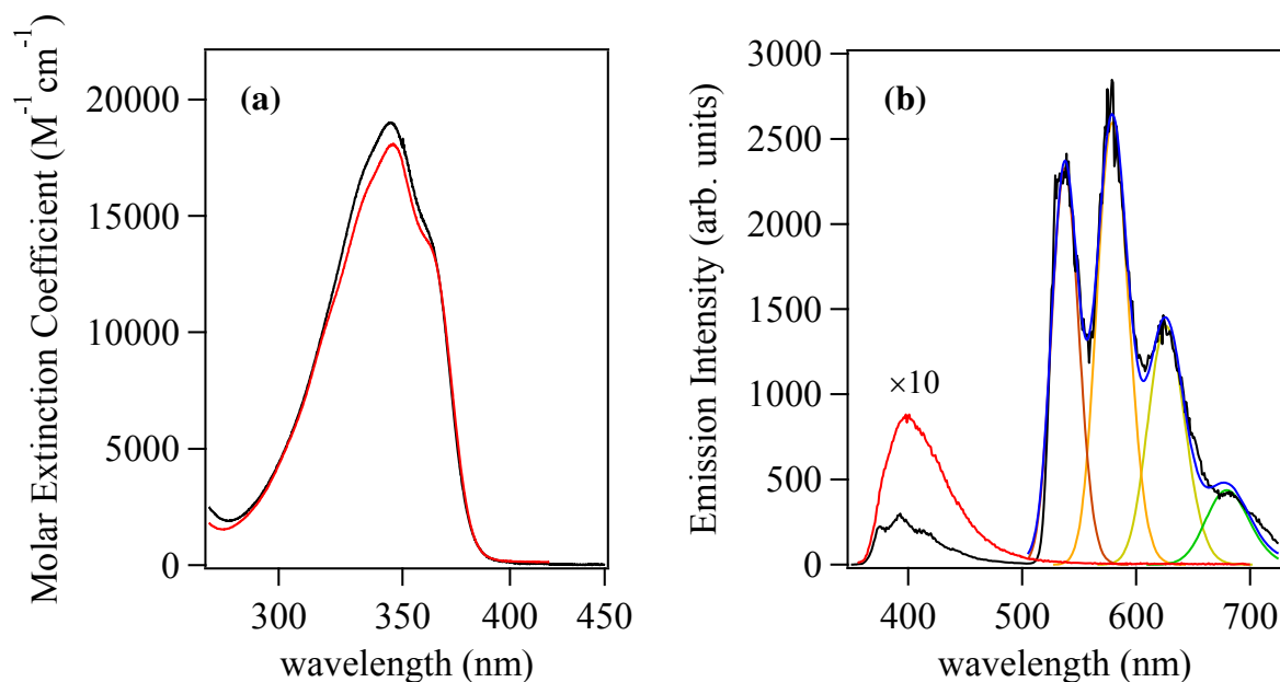
Figure 6. (a) The absorption spectra of the [Yb(5LIO-Me-3,2-HOPO)_2] (red) and [Yb(H(2,2)-Me-3,2-HOPO)] (black) complexes in 0.1 M aqueous TRIS buffer, pH 7.4. (b) Emission spectra ( \lambda_{ex} = 345 nm) at room temperature (red, \times 10 ) and 77 K (black) of the [Gd(5LIO-Me-3,2-HOPO)_2]^- complex measured in a 1:1 (v/v) EtOH:MeOH glassing solvent, and corresponding fit (blue) to a series of overlapping gaussians to evaluate the zero phonon transition.
