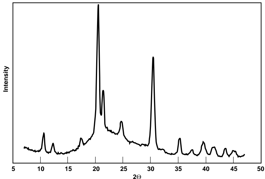
■ Figure 3. X-ray diffraction pattern made by synthetically produced Rb 3 C 60 .
