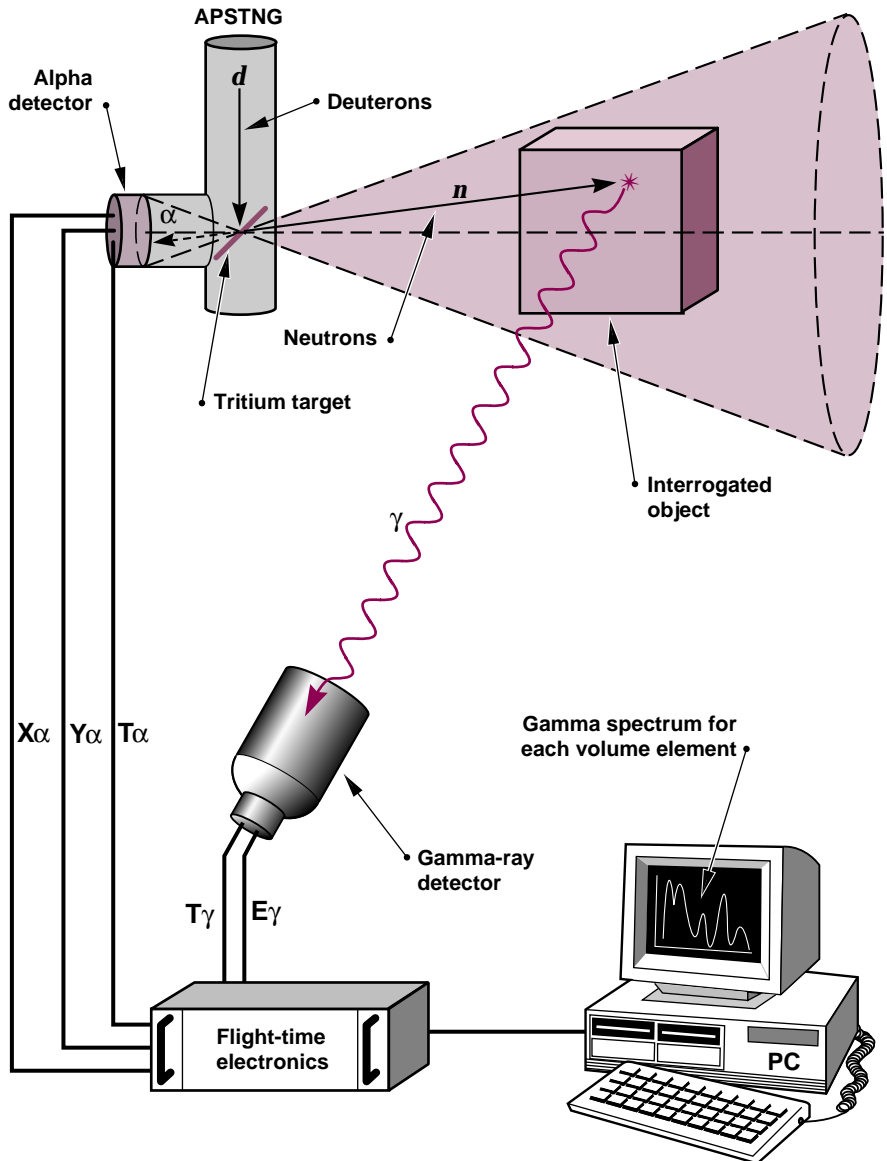
■ Figure 1. Operational layout of the associated-particle, sealed-tube, neutron generator (APSTNG) system.
