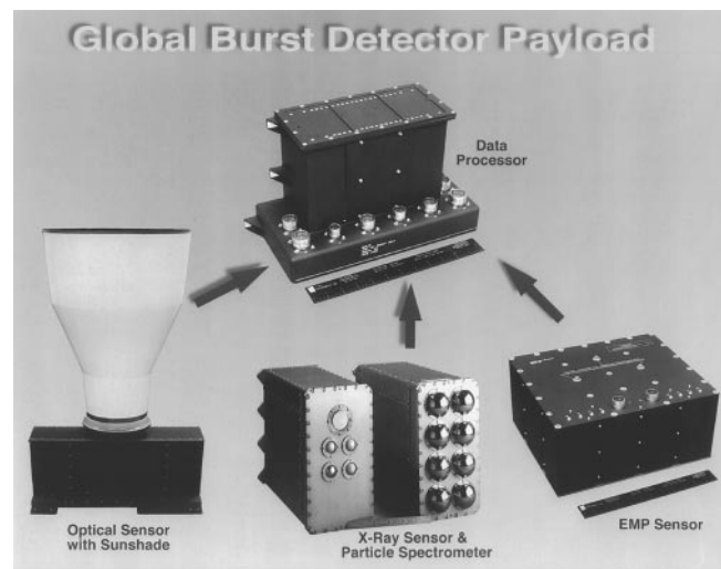
■ Photo 2: The global burst detector (GBD) payload, which consists of a variety of sensors and supporting logic sub-systems and testers.
