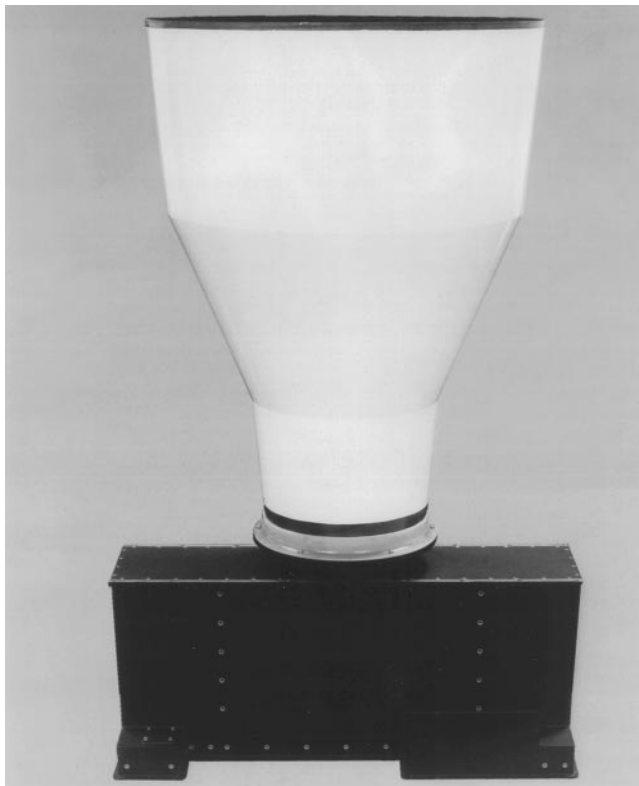
■ Photo 3. The optical sensor is a non-imaging radiometer (bhangmeter) that continuously observes the full-earth disk and responds to the optical signals generated by an atmospheric nuclear detonation. A large, prominent sunshade protects the sensor from sun blinding.
