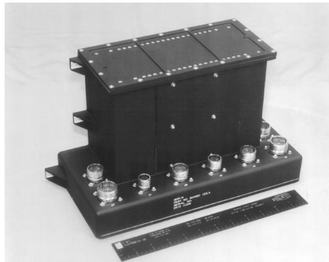
■ Photo 5. The burst detector processor (BDP) processes most NDS functions, including nuclear detonation data. The BDP provides interfaces between the NDS payload and other satellite subsystems; conditions and routes power to the NDS sensors; processes commands and timing information; processes, formats, and stores data; and time tags nuclear events.
