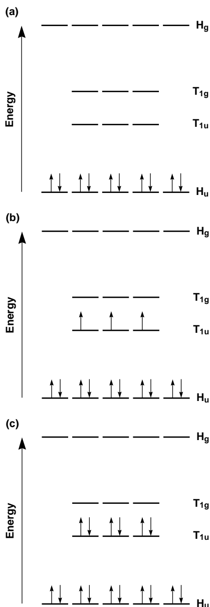
■ Figure 2. The electronic configuration of (a) C 60 , (b) C 60 3- , and (c) C 60 6- .
