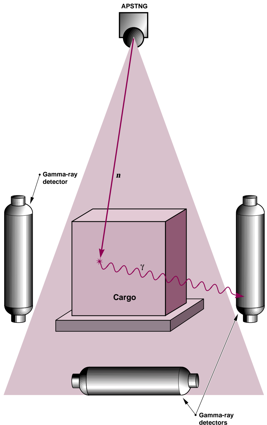
■ Figure 3. Emissive gamma-ray imaging and spectroscopy (EGRIS) APSTNG system proposed for use in detecting special nuclear material (SNM). There are 18 long NaI detectors, each with a photomultiplier on each end (5 detectors are hidden behind each of the 3 detectors shown).
