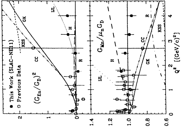
Figure 2. Preliminary neutron form factors, scaled by the dipole fit, along with previous data and theoretical calculations (see text). Error bars include statistical and point-to-point systematic errors.
