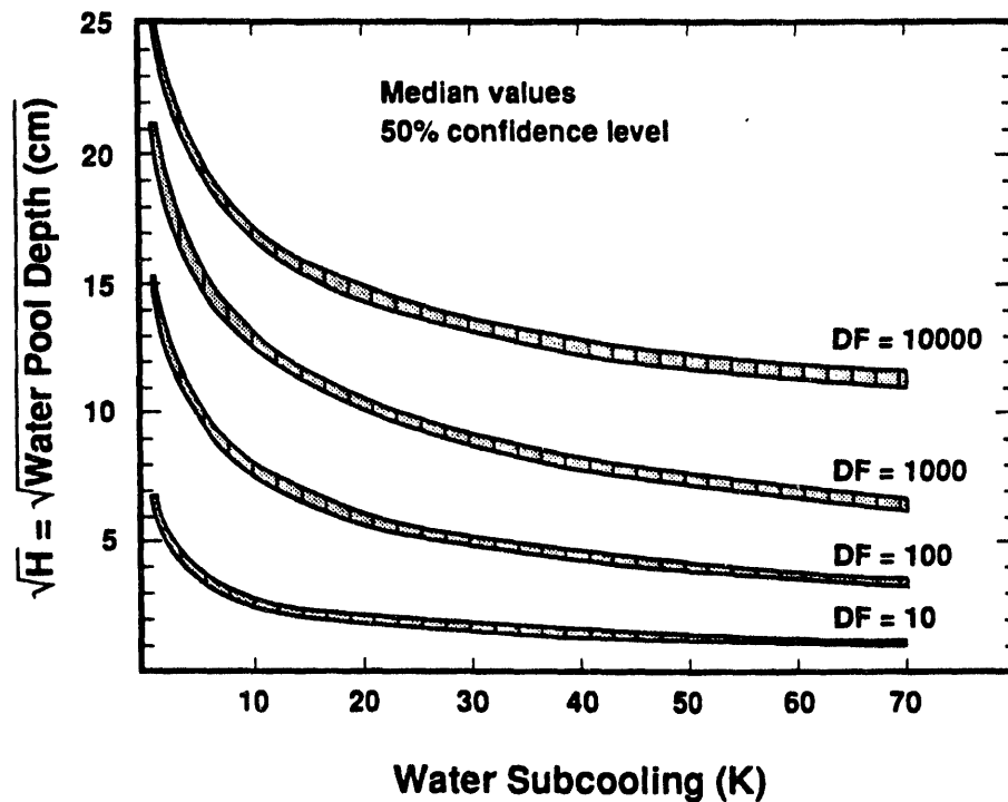
Figure 1 Water subcooling and Depth Needed to Achieve Specified Decontamination of Gases Produced by Core Debris Interactions with Concrete.
