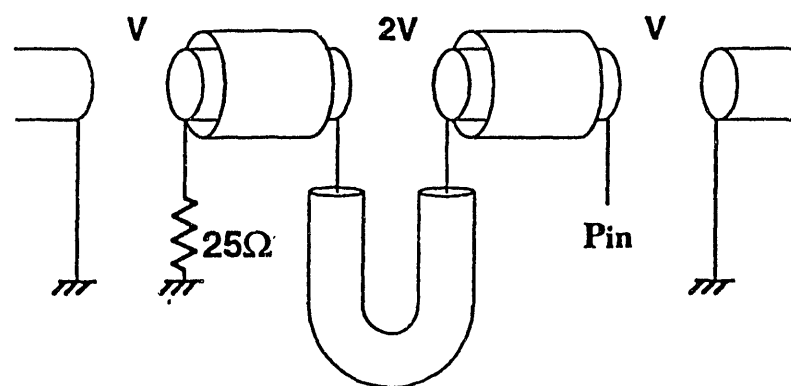
Figure 4: Schematic of Two-Electrode Kicker.
