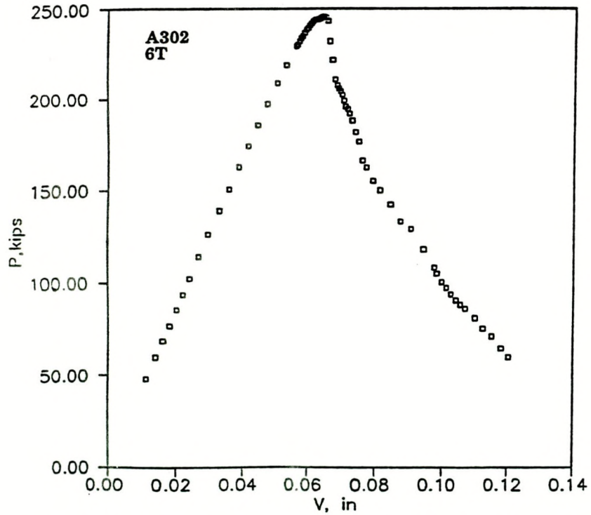
Fig. 8.10 Load vs displacement plot for A 302 steel 6T-CT.
