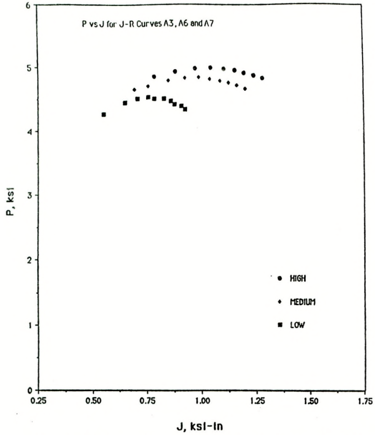
Fig. 7.16. Plot of pressure vs J for A11 model and three weld data J-R curves.
