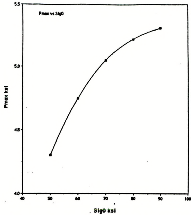
Fig. 7.21. Plot of maximum pressure vs flow stress for A11 model and medium J-R curve.
