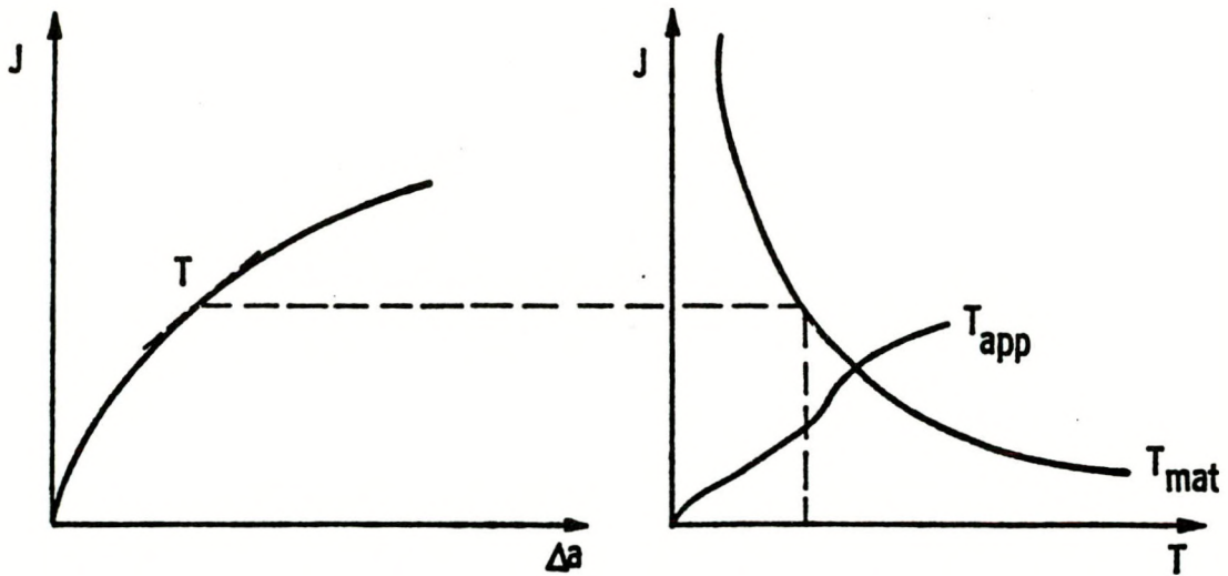
Fig. 3.2 J-T diagram approach to instability prediction.
