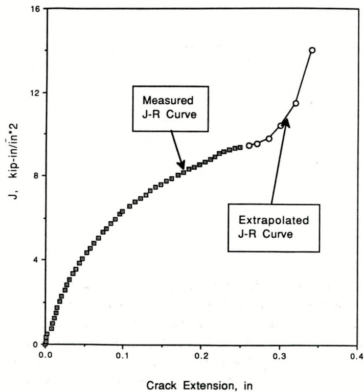
Fig. 6.6 Examples of results from P-v extrapolation, high rise J-R curve.
