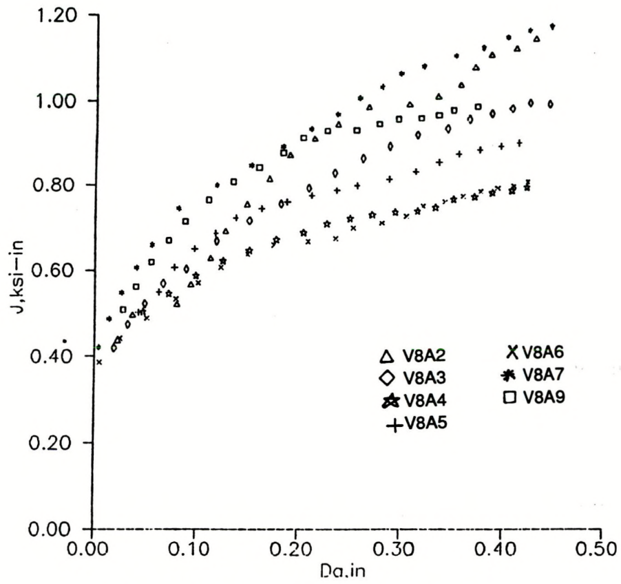
Fig. 7.10 J-R curves for V8A weld data.
