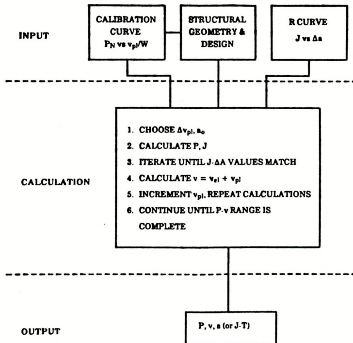
Fig. 3.5 Flow diagram of steps involved in ductile fracture methodology calculations.
