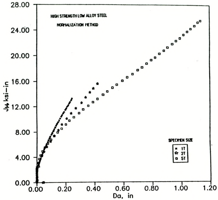
Fig. 5.7 Modified J-R curves for an HSLA steel using normalization analysis.
