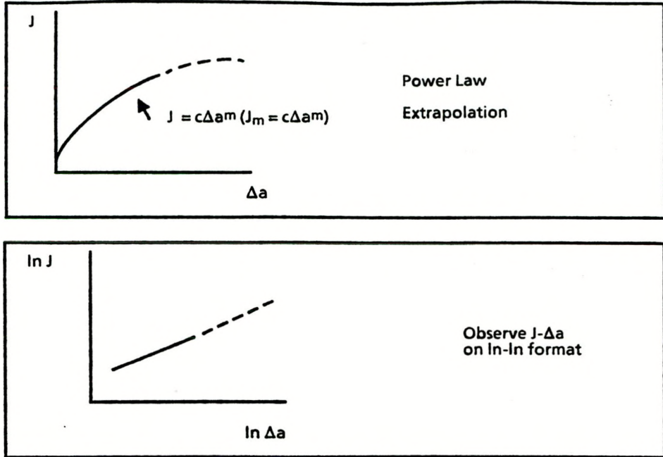
Fig. 6.9 Schematic of direct J-R curve extrapolation ideas.
