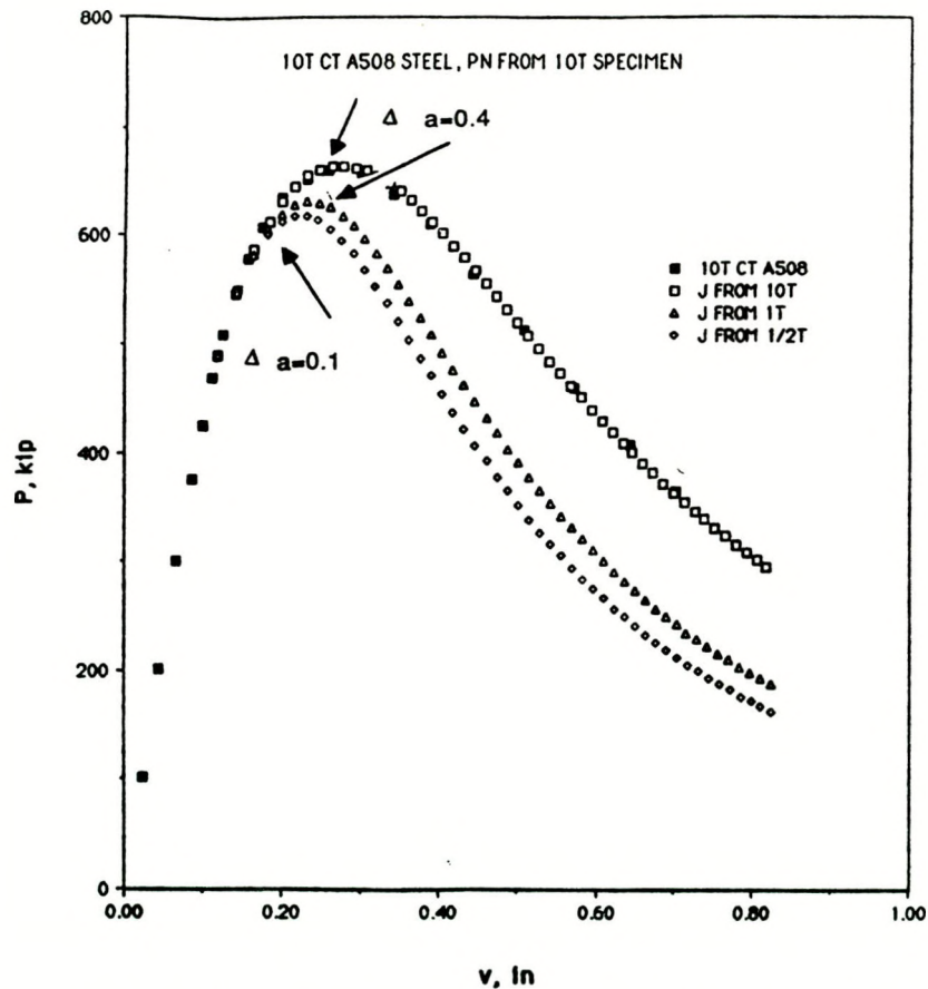
Fig. 9.1. Load vs displacement predictions for A 508 specimens showing 0.1-in. crack extension and crack extension at maximum load.
