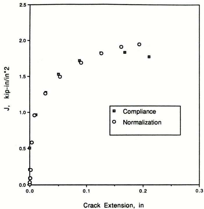
Fig. 4.3. J-R curve for an A 508 steel comparing compliance and normalization measurement of \Delta a .
