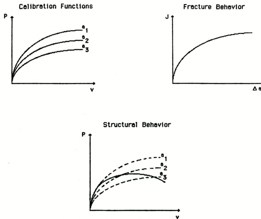
Fig. 3.4. Graphical representation of ductile fracture methodology.
