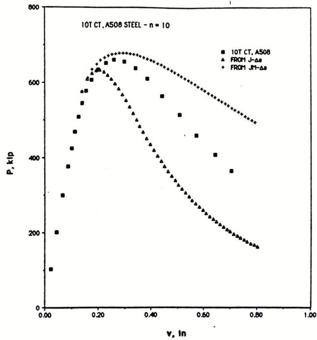
Fig. 7.3. Load vs displacement prediction of 10T-CT from 1/2T-CT J-R curve, A 508 steel.
