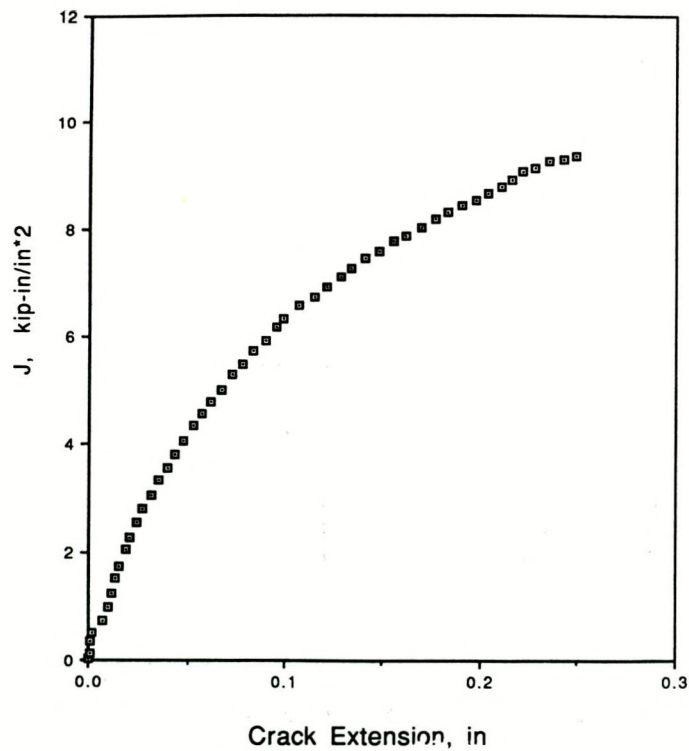
Fig. 6.4 Typical J-R curve from P-v record.
