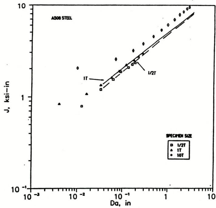
Fig. 7.6. Log-log plot of A 508 J-R curves showing conservative extrapolation.
