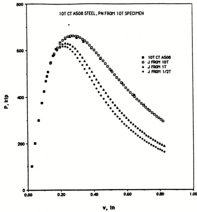
Fig. 7.5. Load vs displacement prediction of 10T-CT varying J-R curves, A 508 steel.
