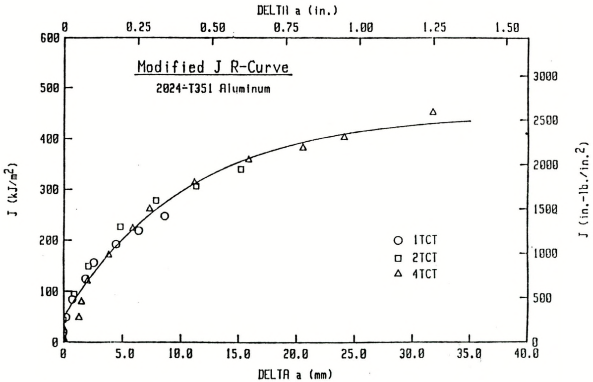
Fig. 5.2 Modified J-R curve for an aluminum alloy eliminating size effect.
