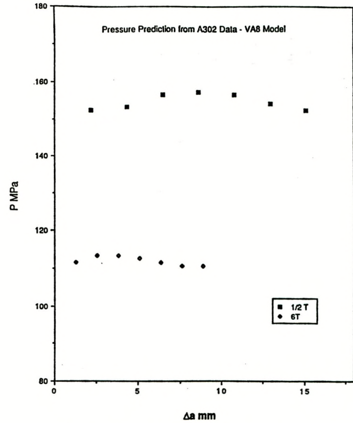
Fig. 8.16. Pressure vs crack extension comparing 1/2T-CT with 6T-CT J-R curve input, V8A ORVIRT model.
