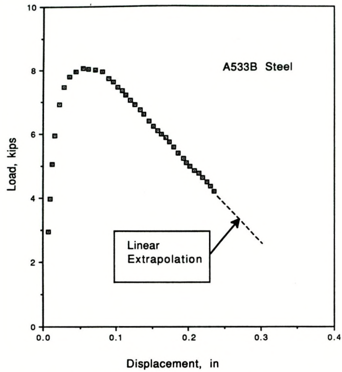
Fig. 6.3 Linear extrapolation of P-v curve.
