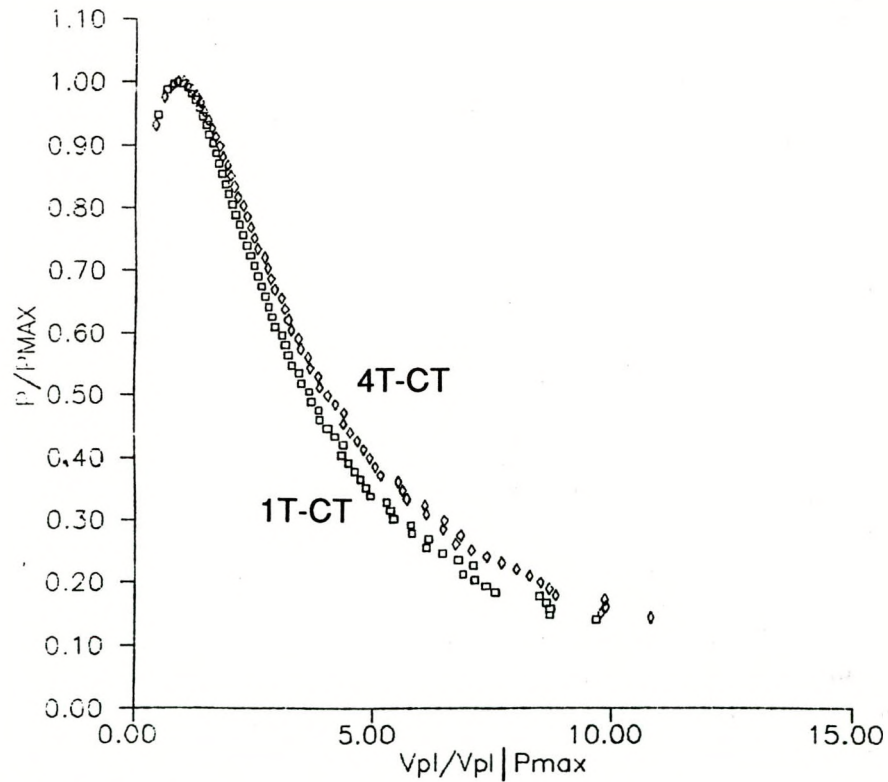
Fig. 6.8 Load vs plastic displacement normalized with maximum load.
