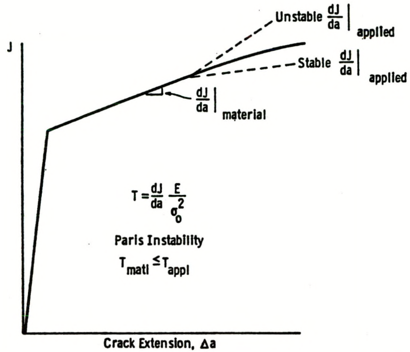
Fig. 3.1 Ductile instability based on the tearing modulus approach of Paris et al.
