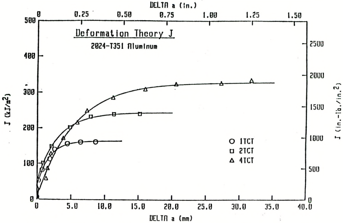
Fig. 5.1 Deformation J-R curves for an aluminum alloy showing size effect.
