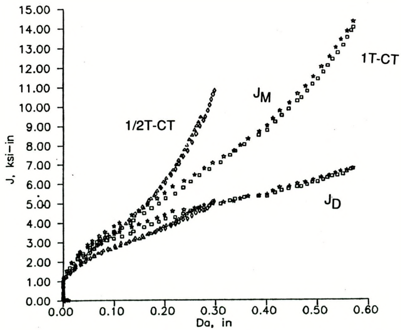
Fig. 5.8 J , J_M -R curves for an A533B steel showing size effect of J_M .
