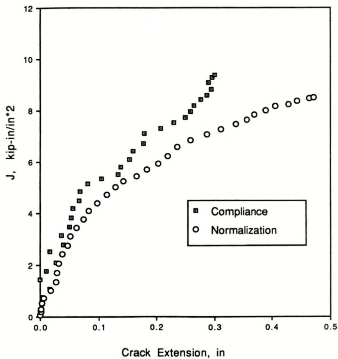
Fig. 4.4. J-R curve for an HSLA steel comparing compliance and normalization measurement of \Delta a .
