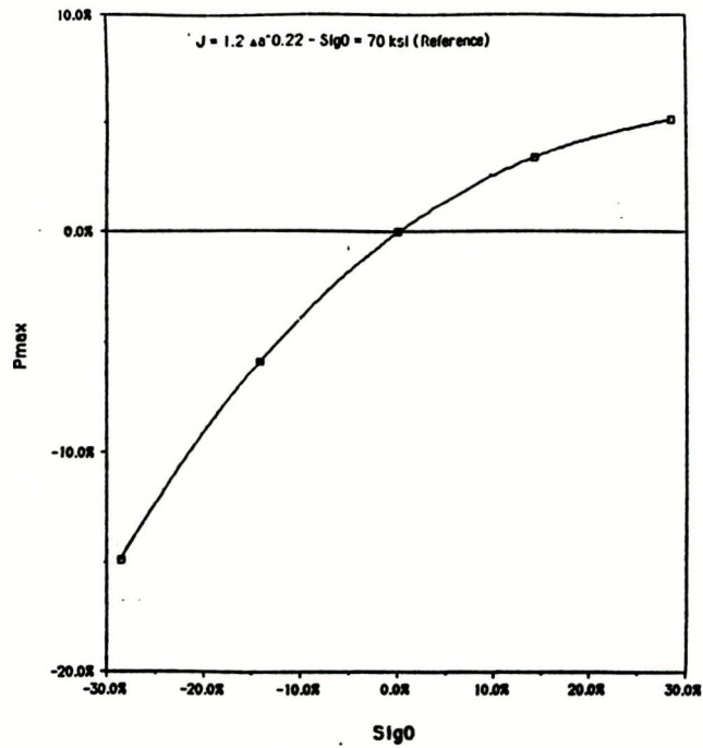
Fig. 7.22. Plot of maximum pressure variation vs flow stress for A11 model and medium J-R curve.
