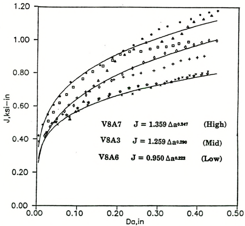
Fig. 7.12. J-R curves for V8A weld data with power-law fits to high, medium, and low data.
