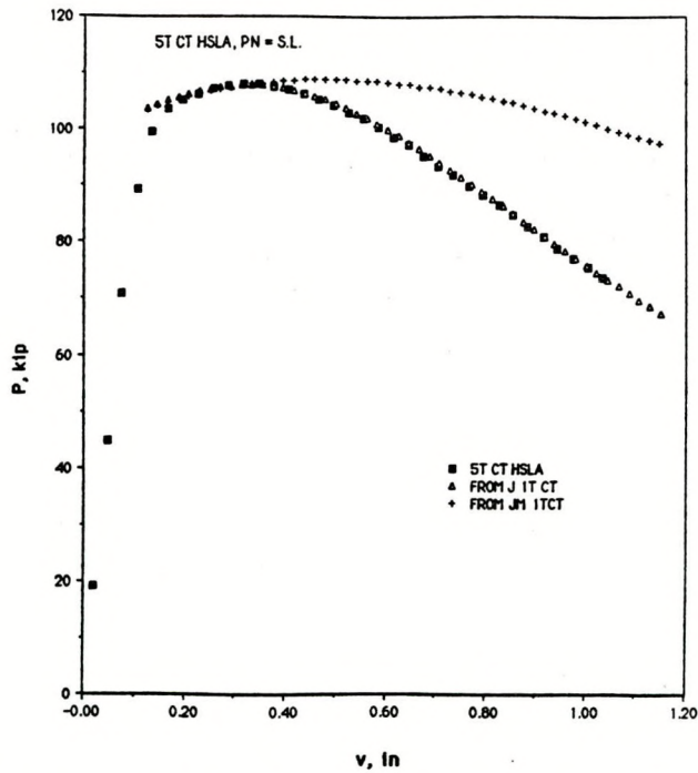
Fig. 7.8. Load vs displacement prediction of 5T-CT from 1T-CT using straight-line calibration functions, HSLA steel.
