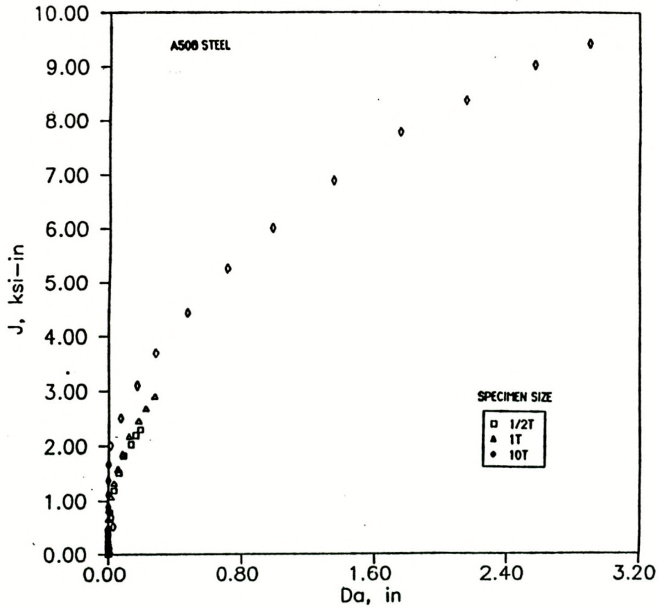
Fig. 5.4 Deformation J-R curve for an A508 steel using normalization analysis.
