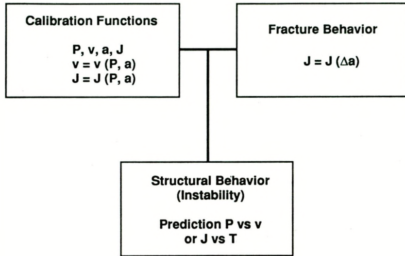
Fig. 3.3. Schematic of ductile fracture methodology based on combining calibration functions with fracture behavior.
