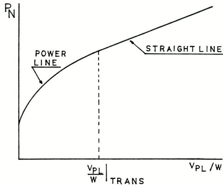
Fig. 7.9. Schematic of normalized load vs plastic displacement showing power-law and straight-line regions.
