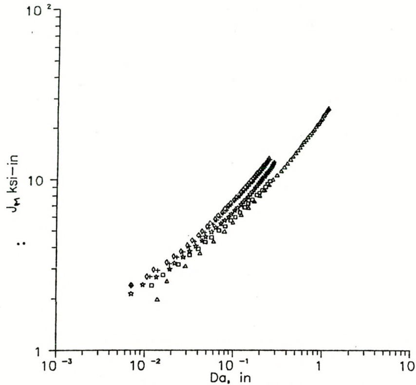
Fig. 6.13. J_M -R curve for HSLA steel on log-log format showing power-law extrapolation.
