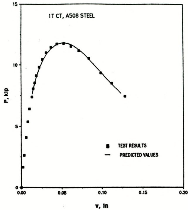
Fig. 3.6. Predictive capability of ductile fracture methodology for A 508 steel.
