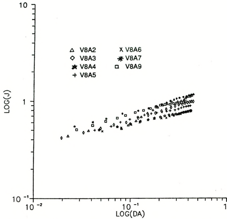
Fig. 7.11. J-R curves for V8A weld data in log-log format.
