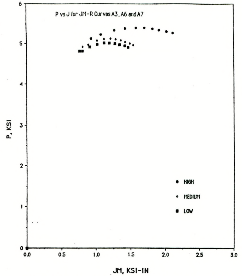
Fig. 7.17. Plot of pressure vs J_M for A11 model and three weld data J-R curves.
