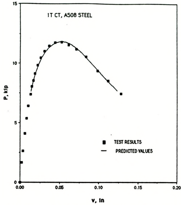
Fig. 7.1. Closed loop prediction of load vs displacement from specimen data for an A 508 steel.
