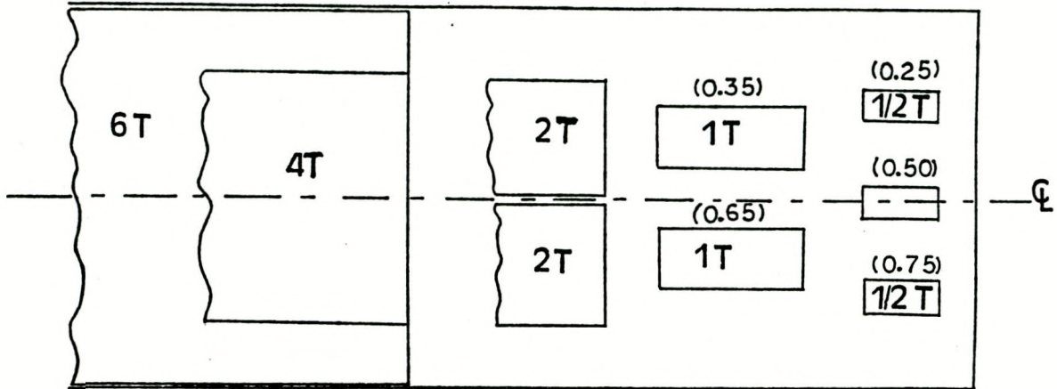
Fig. 8.5. Schematic of A 302 steel plate layout showing through plate thickness of specimens.
