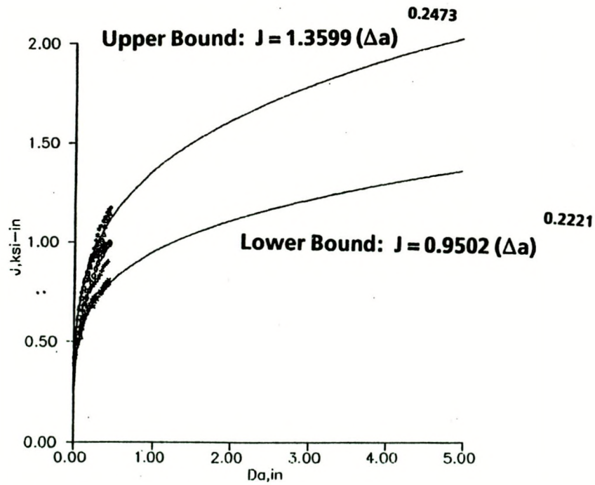
Fig. 7.14. J-R curves for V8A weld data showing extrapolated high and low curves.
