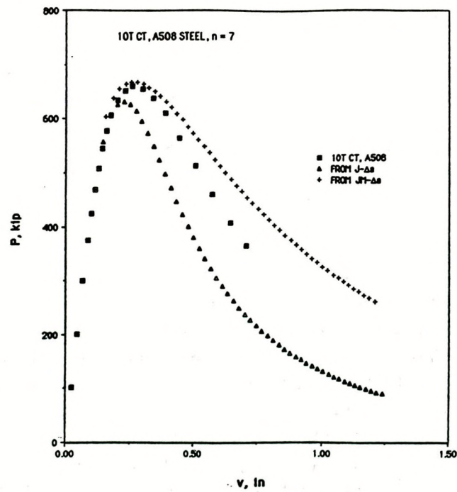
Fig. 7.2. Load vs displacement prediction of 10T-CT from 1T-CT J-R curve, A 508 steel.
