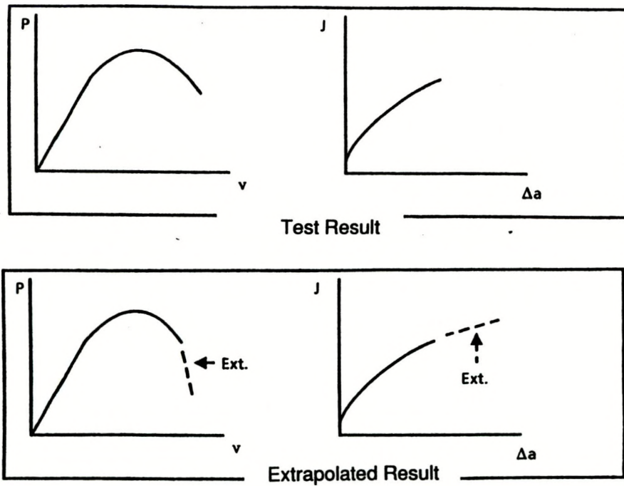
Fig. 6.2 Schematic of J-R curve extrapolation using P-v extrapolation.
