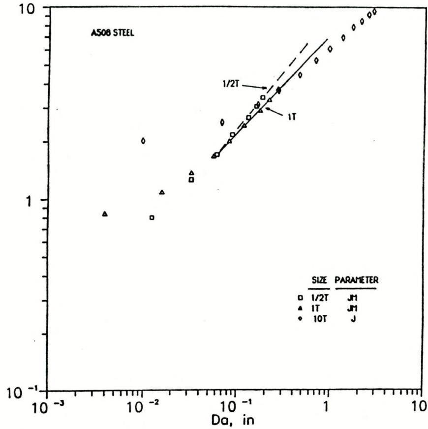
Fig. 6.11 J_M -R curve for A 508 steel on log-log format showing power-law extrapolation.
