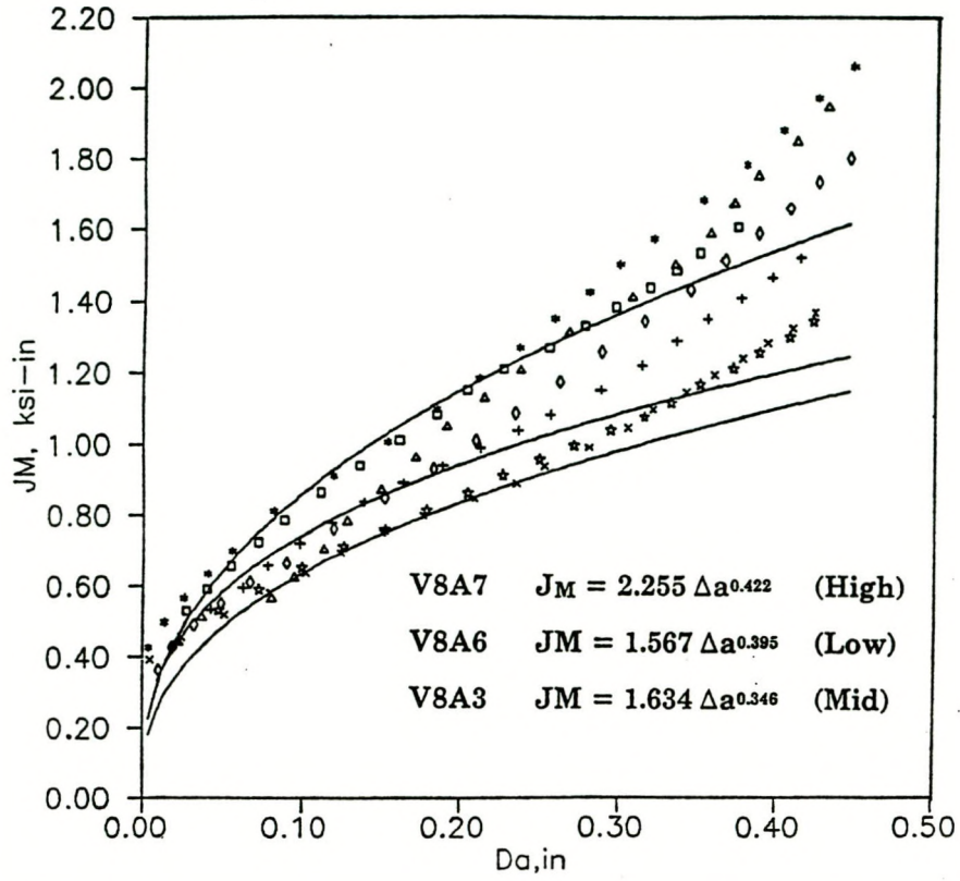
Fig. 7.13. J_M -R curves for V8A weld data with power-law fits to high, medium, and low data.
