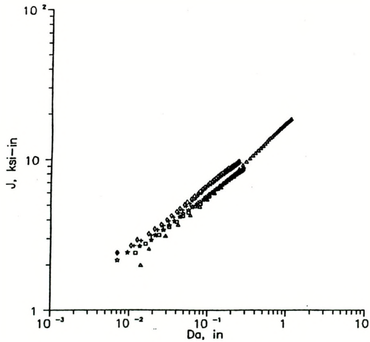
Fig. 6.12 J-R curve for HSLA steel on log-log format showing power-law extrapolation.
