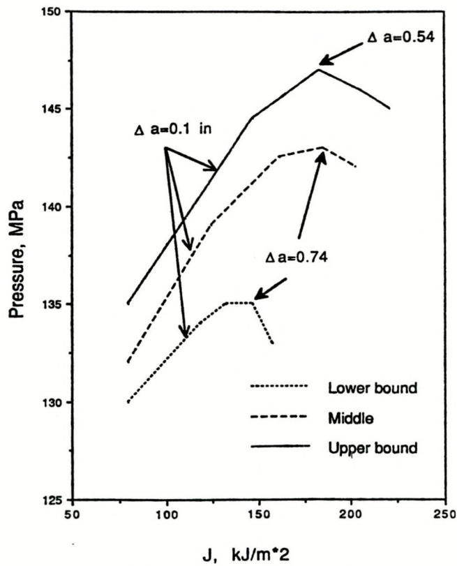
Fig. 9.3. Pressure vs J predictions for V8A weld J-R curves, V8A ORVIRT model showing, 0.1-in. crack extension and crack extension at maximum load.
