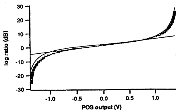
Figure 4. Example of fits to average transfer function.
