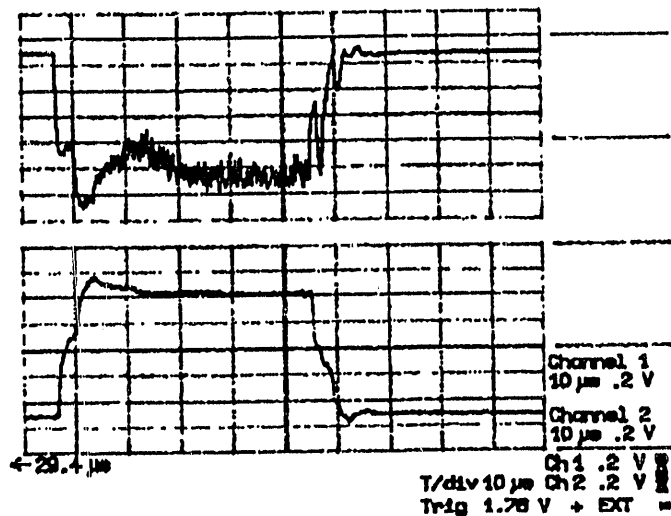
Figure 7. Analog signals: horizontal on top, vertical on bottom. 100mV corresponds to a 1mm displacement.
