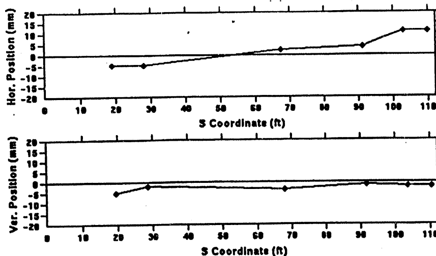
Figure 6. Beam position as displayed on control room console.
