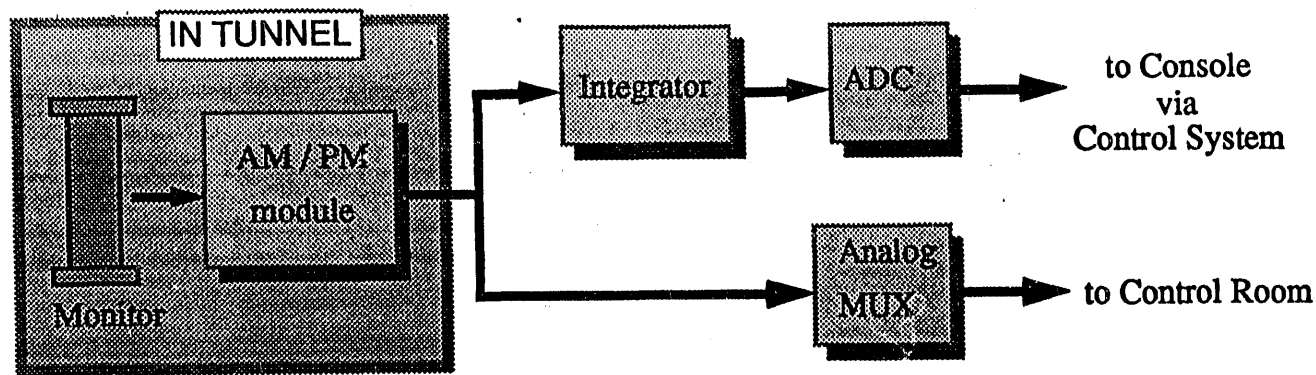
Figure 3. Block diagram of beam position monitoring system.
