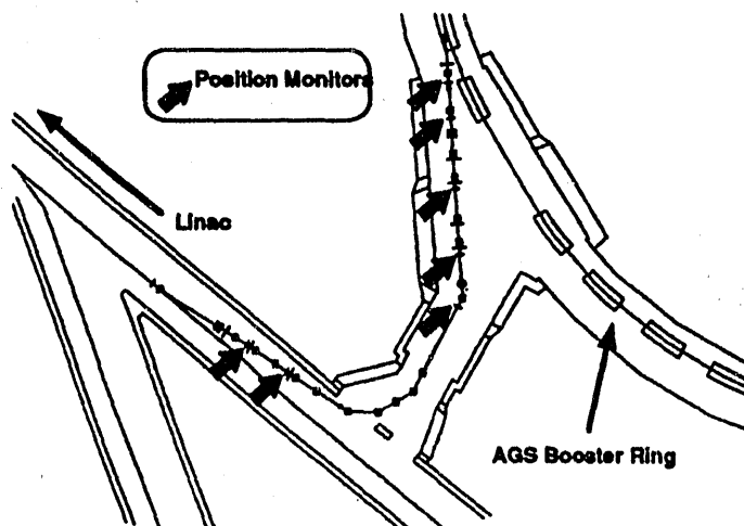
Figure 1. Site Plan.
