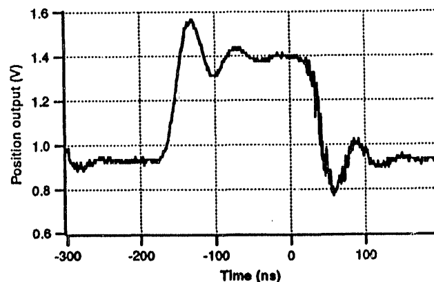
Figure 5. Module's response to simulated beam displacement.
