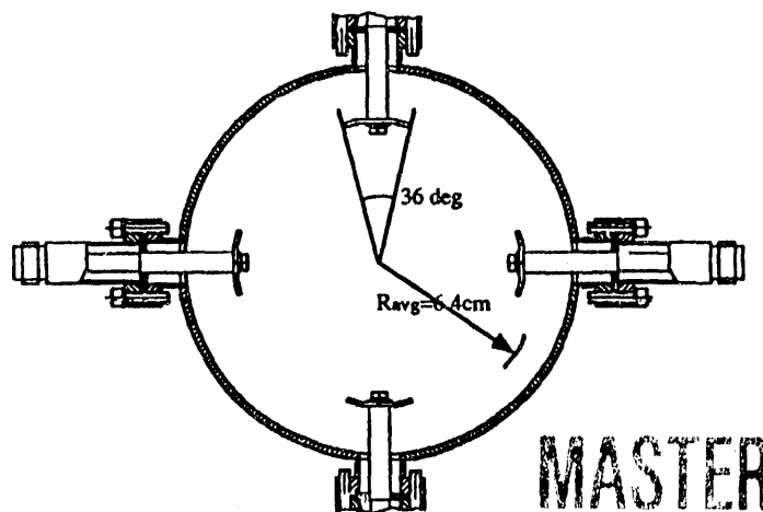
Figure 2. End view of beam position monitor.
