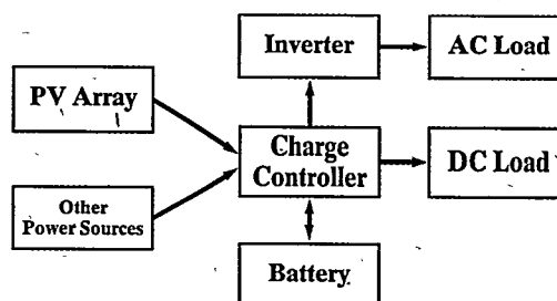
Hybrid system with ac & dc loads, battery, charge controller, & inverter.
