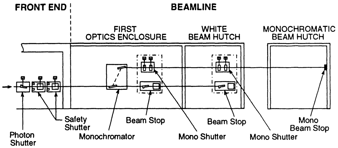
Figure 1. Side view of a possible APS beamline.
