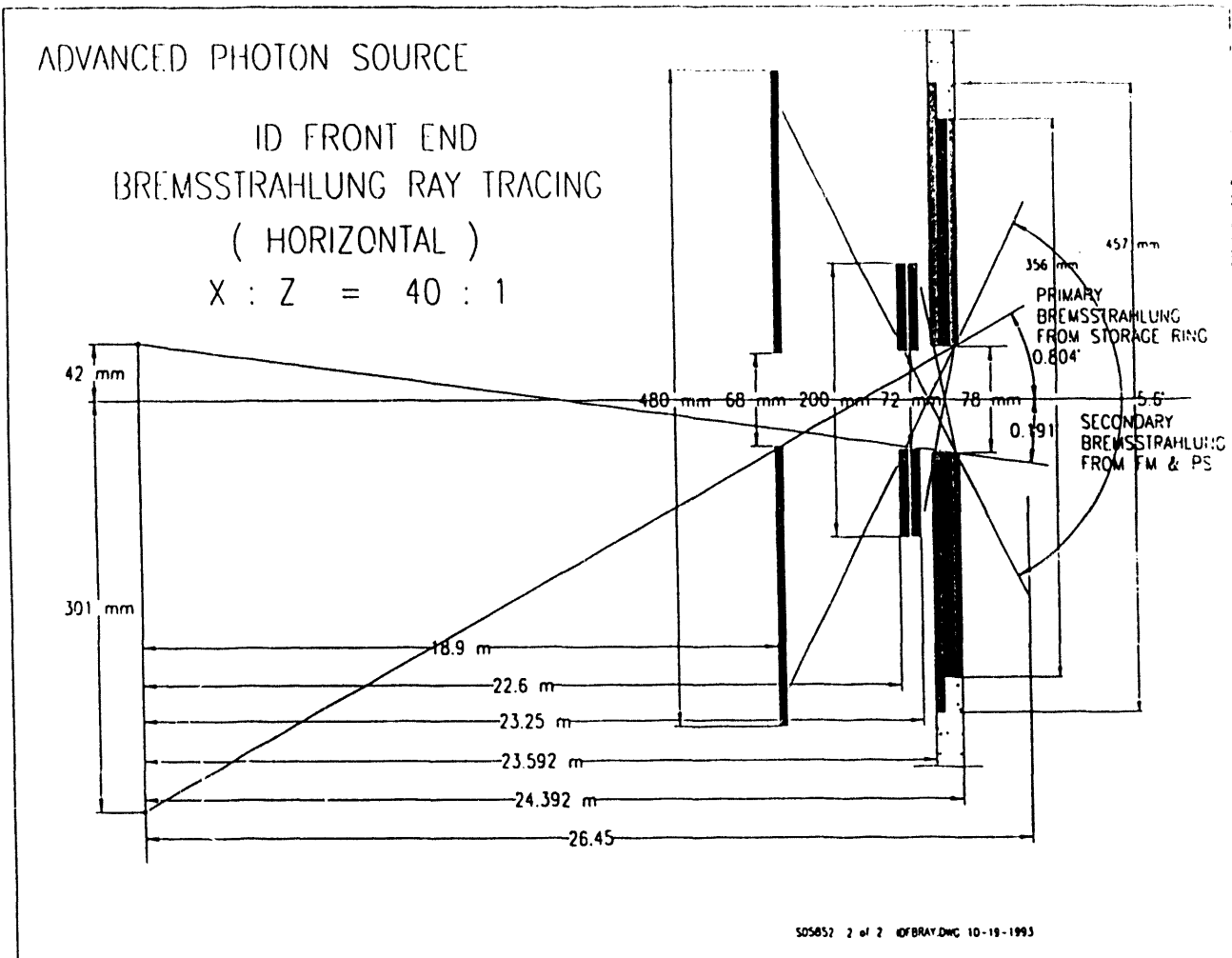
Figure D-2. The bremsstrahlung horizontal ray tracing for the APS insertion device front end.
