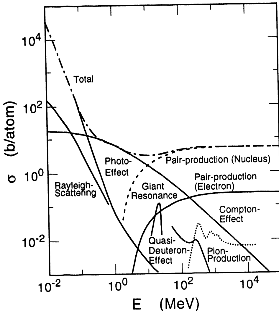
Figure C-2. Photon cross section for Cu. 22
