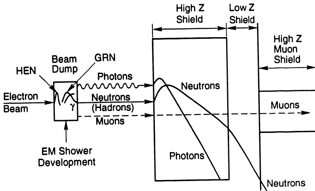
Figure C-3. Typical high-energy electron accelerator shield.
