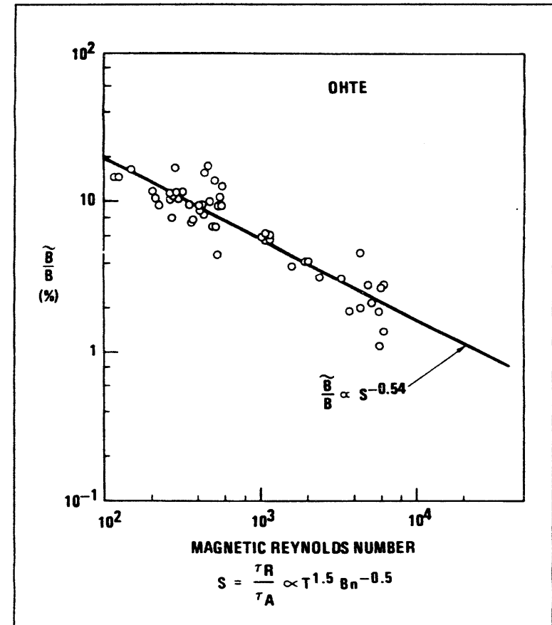
Figure V-3-10) Magnetic fluctuations on OHTE decrease as S^{-0.54} .
