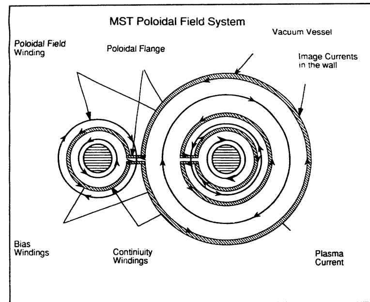
Fig. III-2) Poloidal field system of MST.
