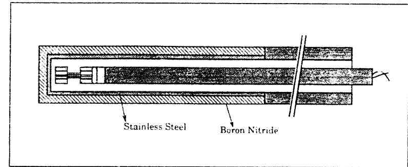
Figure III-10) Assembly drawing for a tri-axial magnetic probe used in this research showing the coils inside the electrostatic shield. The vacuum seal is made on the main probe body and is not shown.
