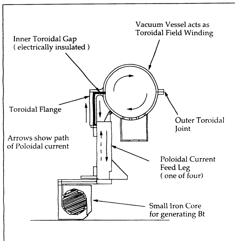
Fig. III-3) Toroidal Field system of MST.
