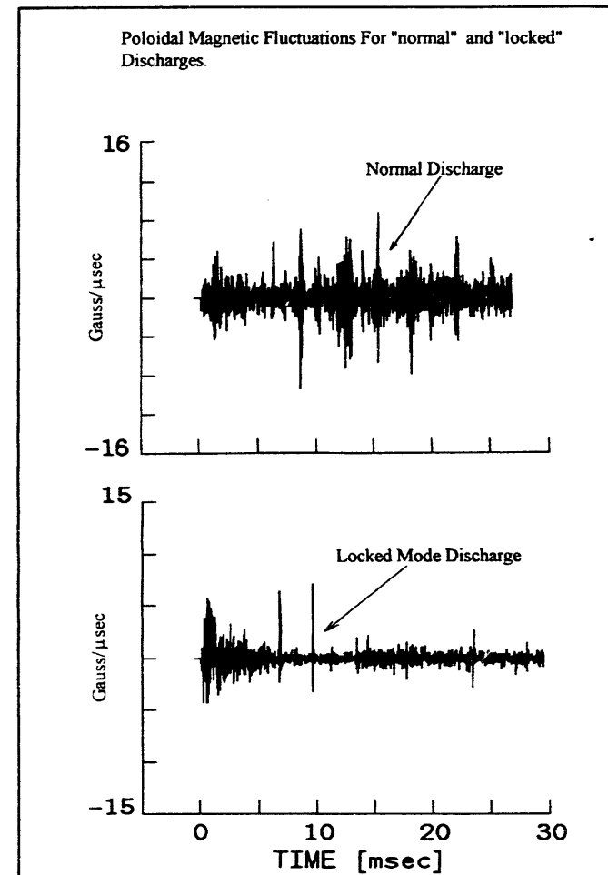
Figure V-2-2) Raw poloidal magnetic fluctuations measured. High fluctuations are present when discharges are "normal" ( top Fig.). Mode locking occurs, in the bottom Fig. at 5.3 ms.
