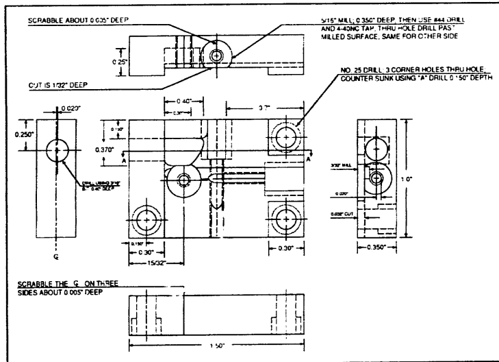
Figure III-5) Schematic drawing of a fixed coil set which are installed on inside wall of MST.
