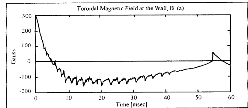
Figure 1-1) Self-generation and sustainment of toroidal field measured at the edge of MST. Sawtooth oscillations are observed.
