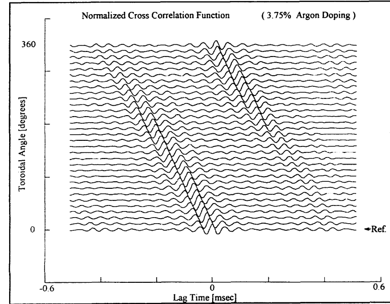
Figure V-8-5) Toroidal cross-correlation of edge magnetic fluctuations. Coherent modes exhibit "slowing down" when impurities (3.75% argon doping) are added to hydrogen plasmas.
