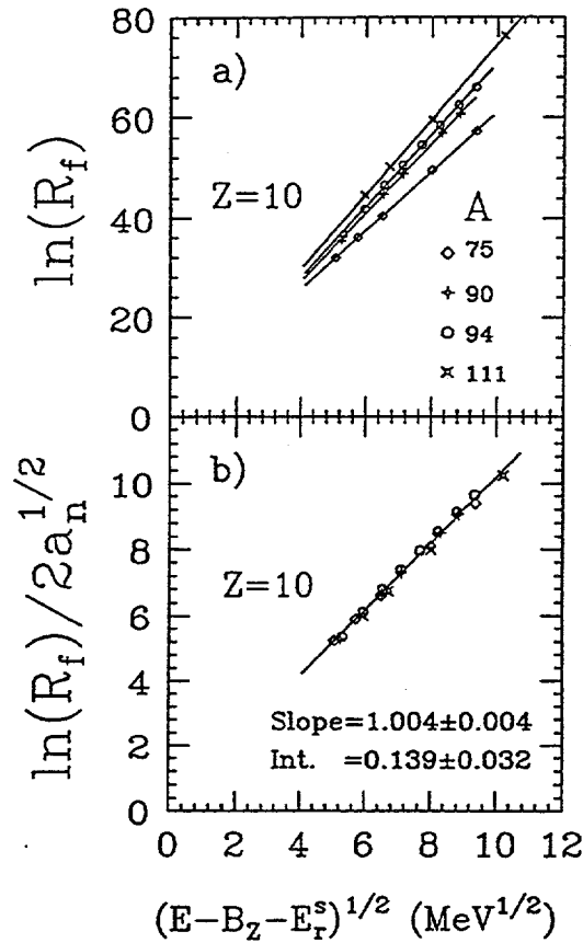
Fig. 3. \ln R_f a) and \ln R_f/2a_n^{1/2} b) vs the intrinsic excitation energy for Z = 10 fragments from the compound nuclei: ^{75}\text{Br} , ^{90}\text{Mo} , ^{94}\text{Mo} , and ^{110,112}\text{In} . The A -dependence of R_f vs a_n is shown in a), while this A -dependence is removed in b).
