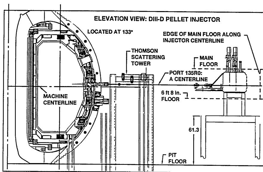
Figure 1. Schematic of three-barrel injector installation on DIII-D.
