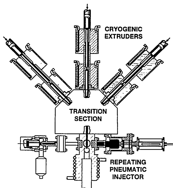
Figure 4. Schematic of steady-state extruder feed system; three standard extruders operate in tandem to provide a continuous source of frozen hydrogen.
