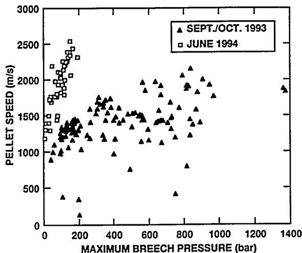
Figure 2. Experimental data from a repeating two-stage light light gas gun (ORNL/Frascati collaboration)
