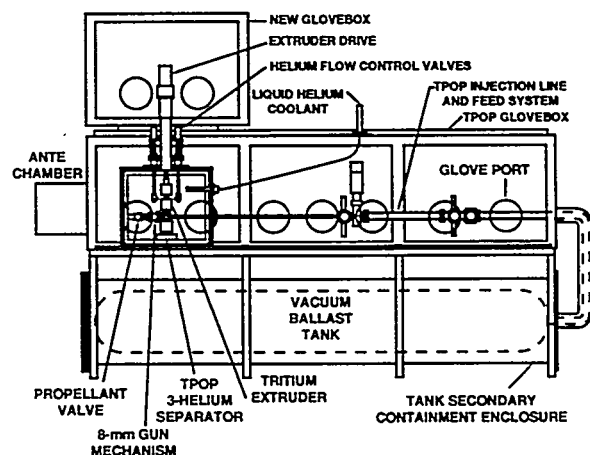
Figure 3. Schematic of TPOP II experiment.
