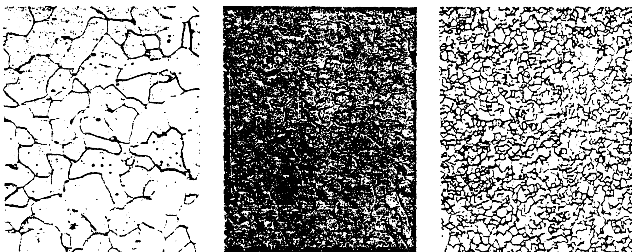
Figure 2. Microstructures of commercial SAE 1008 hot band (left), as-deposited spray-formed strip (center), and hot-rolled spray-formed strip (right). 400X
