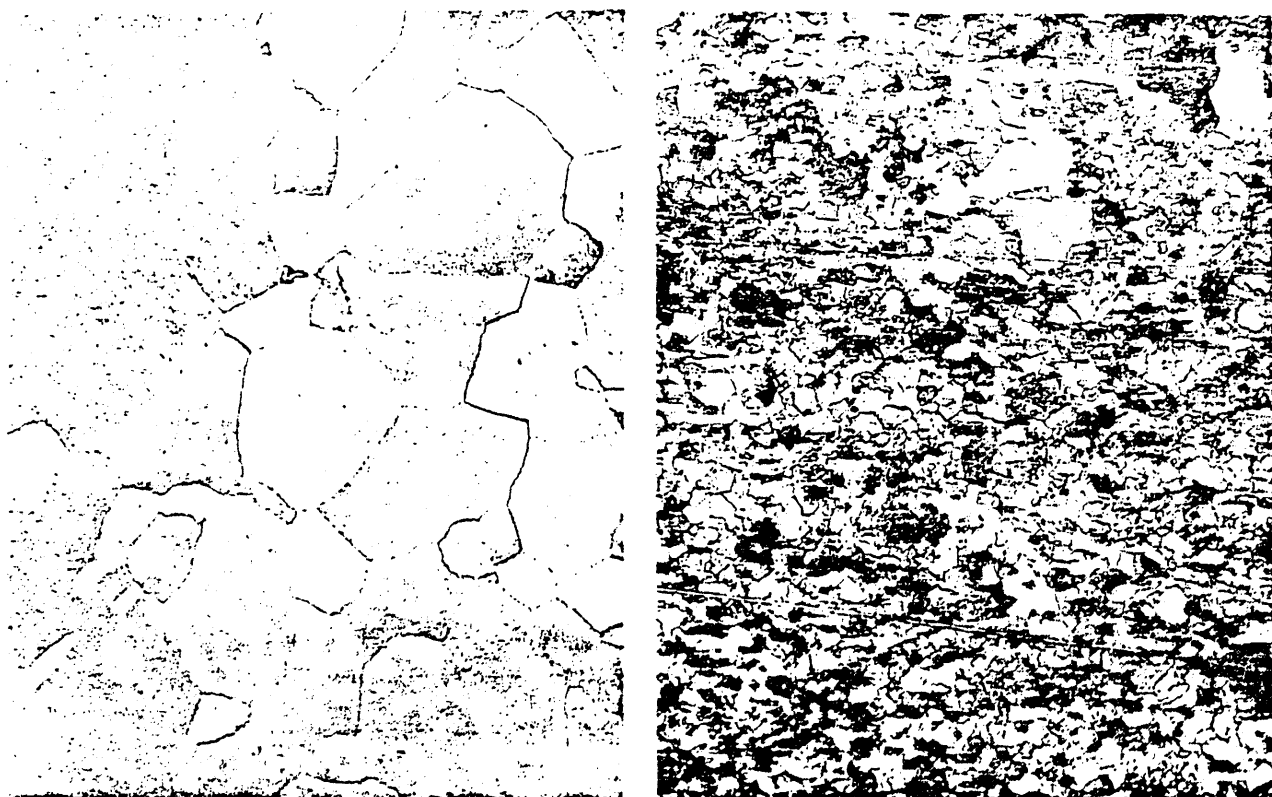
Figure 7. Microstructures of cast tin (left) and spray-formed tin mold of Figure 6 (right). 400X
