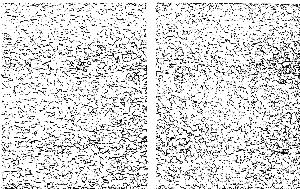
Figure 4. Microstructure of SAE 1008 steel hot band (left) and thick ( >\sim 9 mm) spray-formed and hot-rolled strip (right). 100X
