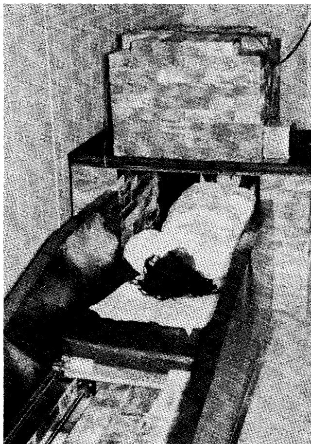
Arrangement of lead bricks used for whole-body counting.
