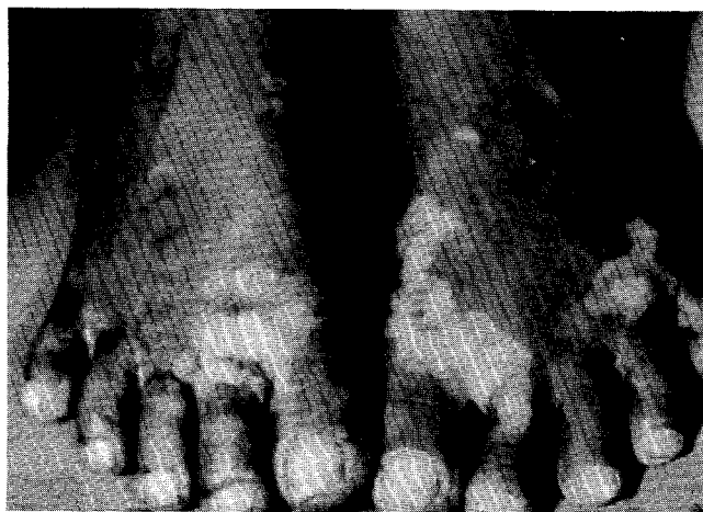
Radiation burns of the feet.
