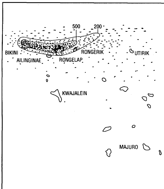
Fallout area in the Marshall Islands.
