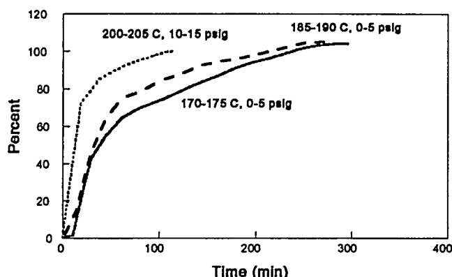
Fig. 4. Oxidation of Polyethylene
