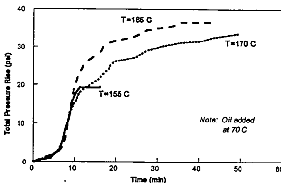
Fig. 3. Trimsol Oxidation at Maximum Nitric Acid Conditions
