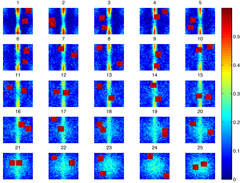
(a) Visualization of the tensor \tilde{\mathbf{X}}'' : combined artifact and Gaussian noise in each slice (Intensity of pixel ijk is \log(1 + x_{ijk}) ).
