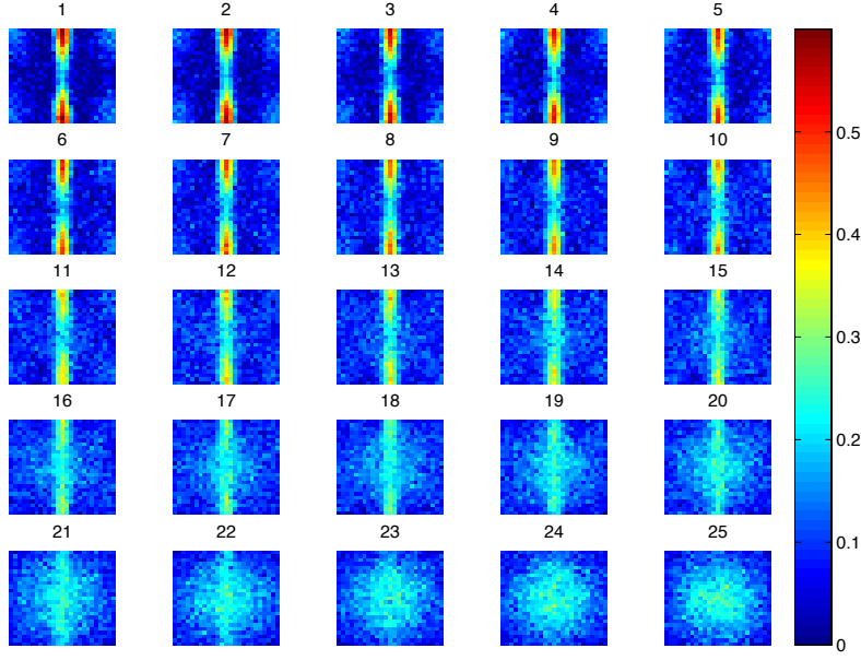
(a) Visualization of the tensor \tilde{\mathbf{X}} : Twenty five frontal slices size 25 \times 25 with Gaussian noise (Intensity of pixel ijk is \log(1 + x_{ijk}) ).
