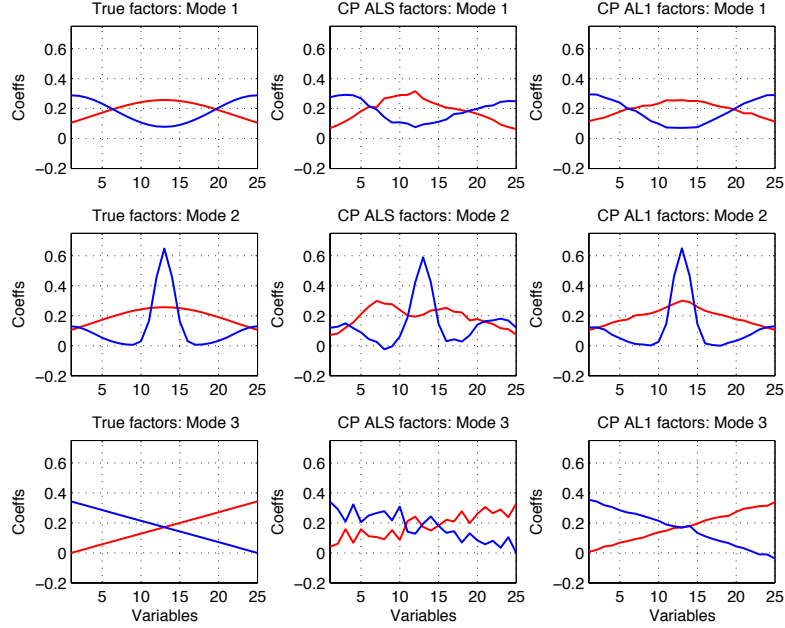
(b) The rank two CPALS factorization continues to diverge from the true factorization as more non-Gaussian perturbations add added and Gaussian noise is also added to all entries. The two CPAL1 factorization still agrees with the true factorization.
