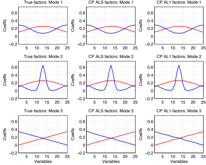
(b) Rank two CP factorizations of \tilde{\mathbf{X}} by CPALS and CPAL1 agree with each other and the true generative factorization.
