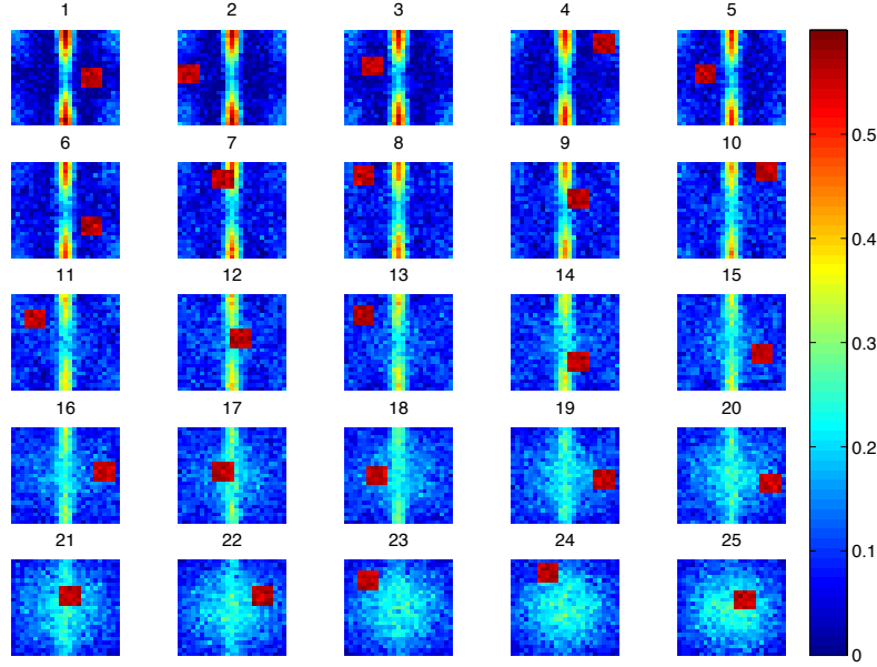
(a) Visualization of the tensor \mathfrak{X}' : combined artifact and Gaussian noise in each slice (Intensity of pixel ijk is \log(1 + x_{ijk}) ).
