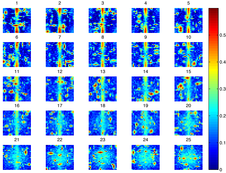
(a) Fifty pyramids with randomly assigned height, location, and base are placed in each frontal slice of \mathfrak{X} and Gaussian noise superposed afterward (Intensity of pixel ijk is \log(1 + x_{ijk}) ).
