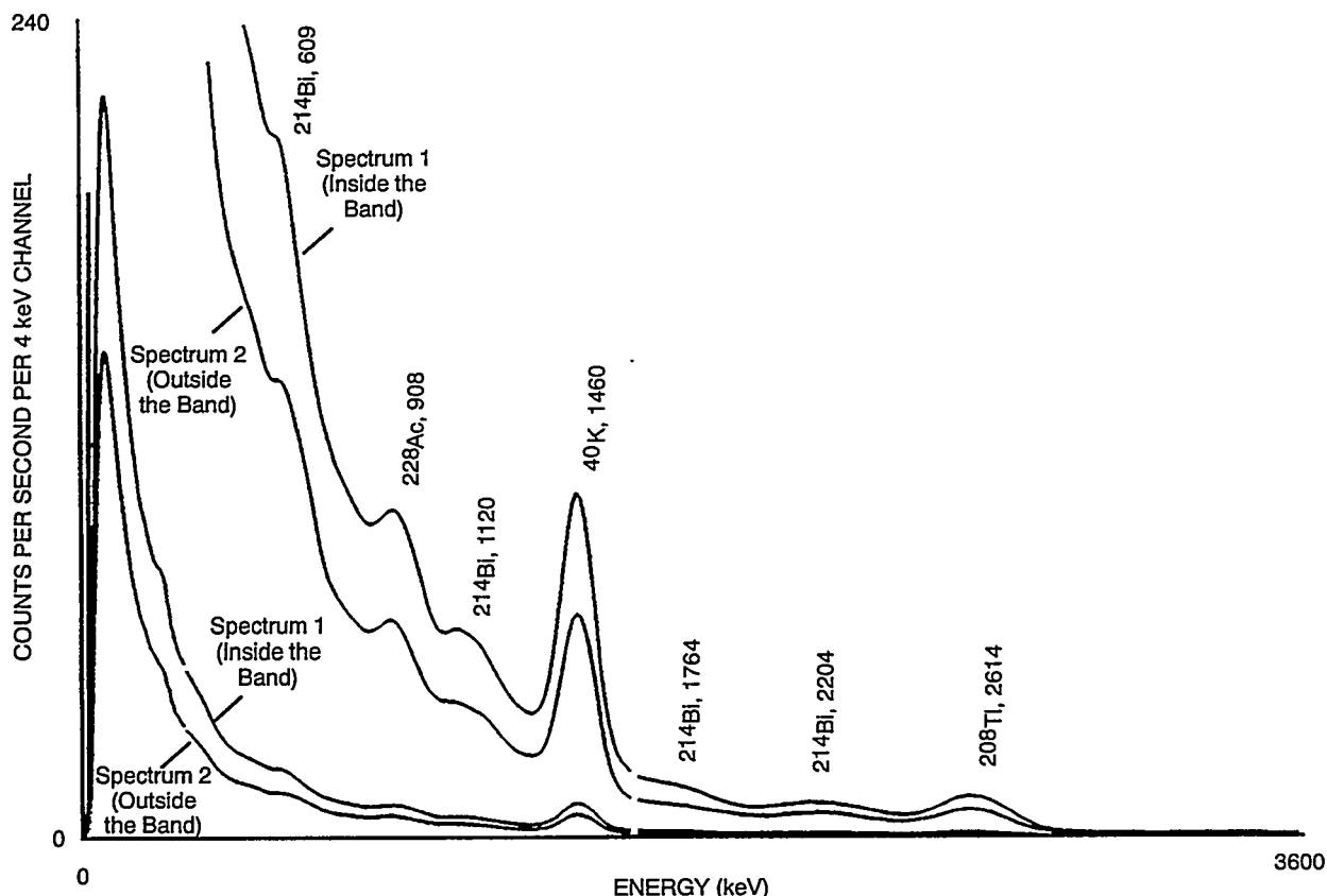
FIGURE 3. SPECTRA MEASURED INSIDE AND OUTSIDE THE BAND OF ELEVATED ACTIVITY. Two curves are shown for each spectrum, differing in scale by 10.
