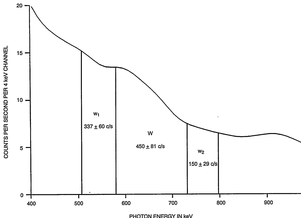
FIGURE 4. CESIUM-137 SPECTRAL WINDOWS. The count rate shown in each window is the average of approximately 200 one-second measurements taken over the test line plus/minus the standard deviations. These standard deviations are several times what would be expected from counting statistics alone, the increase being due to real fluctuations in natural radioactivity.
