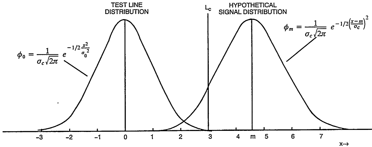
FIGURE 5. DISTRIBUTION FOR SIGNAL = 0 AND SIGNAL = m
