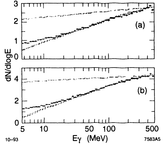
Figure 7: The observed bremsstrahlung spectrum dN/d\log E (crosses) for two uranium targets, in units of photons per bin per 1000 electrons, for a 2% X_0 (a) and 5% X_0 (b) thick target. The dotted line (top) shows the Bethe-Heitler Monte-Carlo expectation, whereas the dashed line (bottom) is the Monte-Carlo expectations including the LPM effect.
