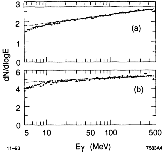
Figure 6: The observed bremsstrahlung spectrum dN/d\log E (crosses) for two carbon targets, in units of photons per bin per 1000 electrons, for a 2% X_0 (a) and 6% X_0 (b) thick target. The dotted line (top) shows the Bethe-Heitler Monte-Carlo expectation, whereas the dashed line (bottom) is the Monte-Carlo expectations including the LPM effect. The solid line (top) in (a) is the Bethe-Heitler prediction ignoring multi-photon pileup.
