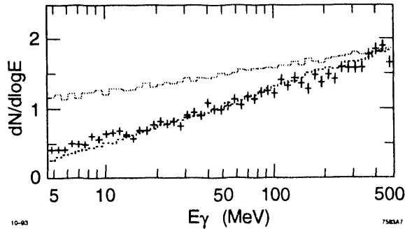
Figure 8: The difference between the bremsstrahlung spectra for the two uranium targets, with observed and expected spectra. Obtained by subtracting Figure 7(a) from Figure 7(b).
