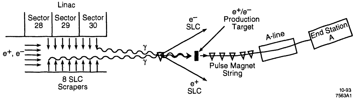
Figure 4: A diagram of the parasitic beam generation. High energy photons produced in the collimators of sectors 28–30 travel downstream, past the bending magnet that directs electrons and positrons into the SLC arcs, and onto an e^+e^- production target in the beam switchyard. Electrons produced in the target are captured by the A-line and transported to End Station A.
