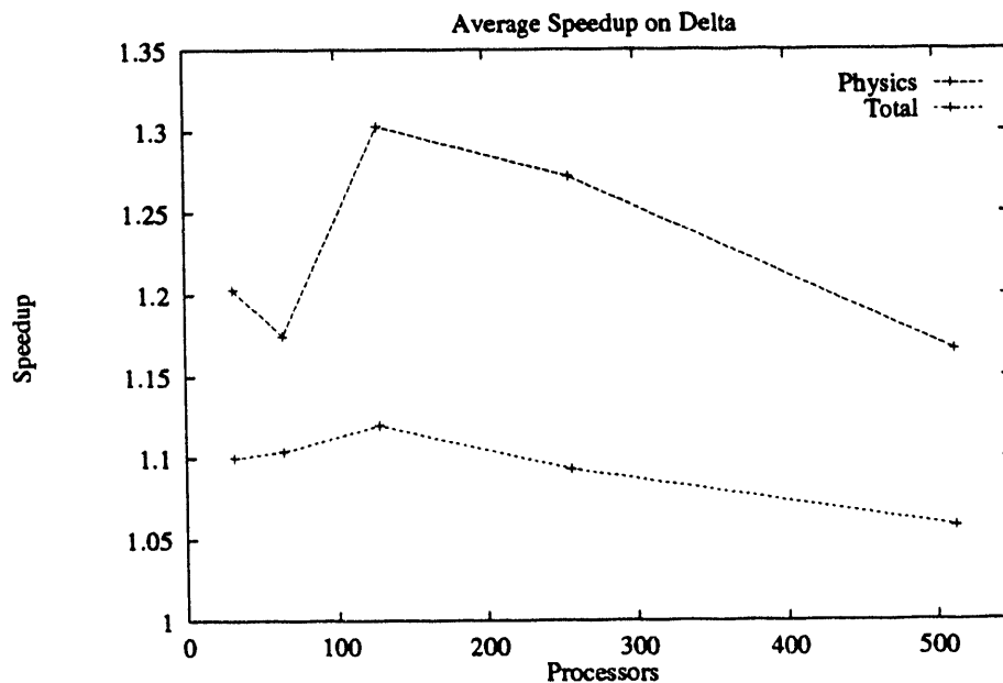
Figure 3: Speedups from load balancing
