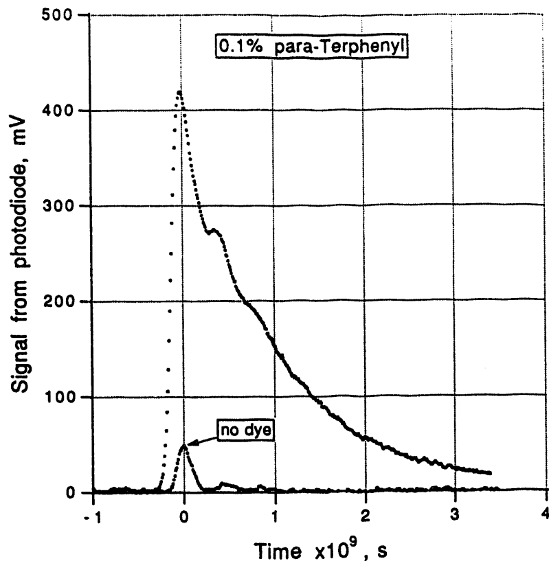
Figure 3. Fluorescence transient from silica sol-gel containing 0.1% p-terphenyl after excitation by a 30 ps pulse of 20 MeV electrons. The lower trace shows the Cerenkov light generated in a sol-gel sample without dye.
