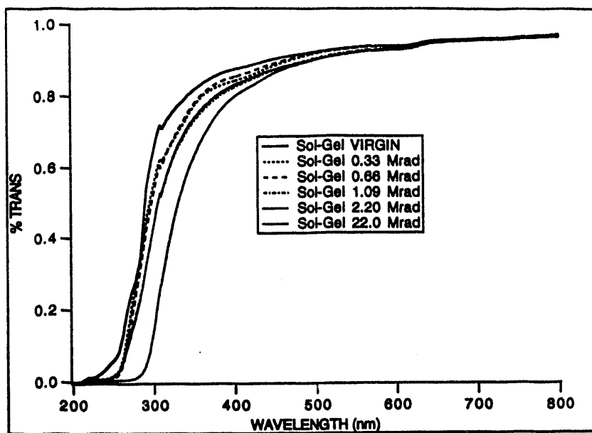
Figure 1. Transmission spectrum of silica sol-gel as a function of radiation dose ( ^{60}\text{Co} \gamma -rays, 0.4 Mrad/h).
