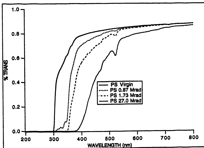
Figure 2. Transmission spectrum of polystyrene (PS) as a function of radiation dose ( ^{60}\text{Co} \gamma -rays, 0.4 Mrad/h).
