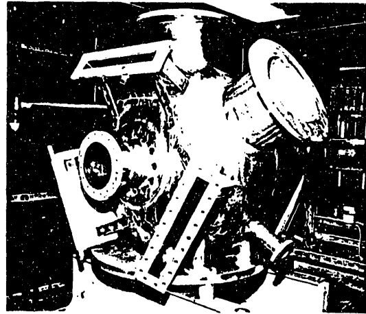
Fig. 2. PEP-II low-power cavity prototype.
