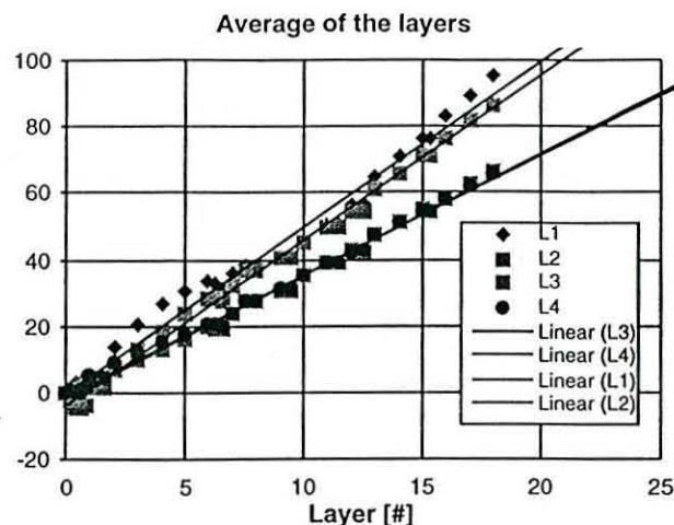
Figure 1 Winding layer Load versus stretched wire layer #
