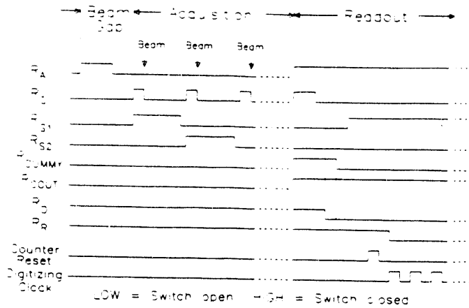
Fig. 3. Timing diagram
