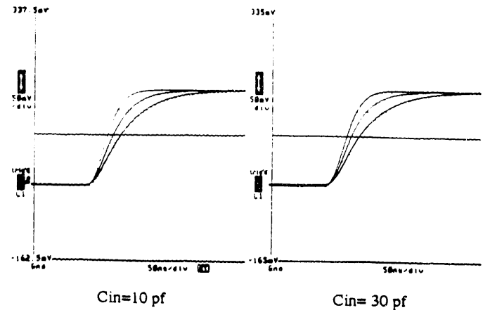
Fig. 4. Measured system risetime
