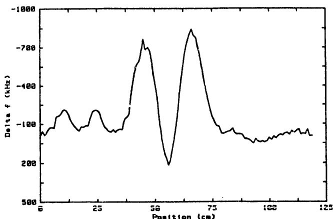
Figure 2c: Trapped Dipole.
