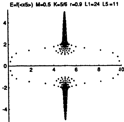
Figure 4. The energy spectrum as a function of the average position in the extra dimension on a N_1 = 24 by N_5 = 11 lattice. Note how the low energy modes lie near the ends of the lattice.
