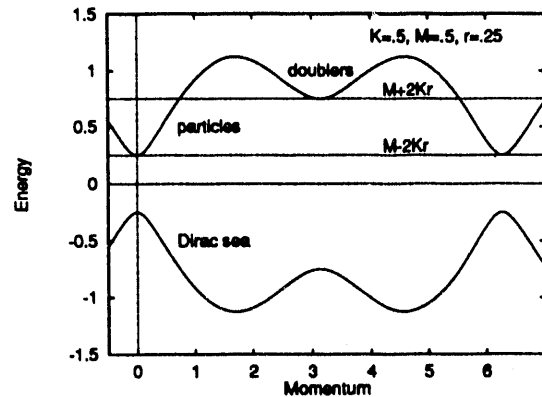
Figure 1. The spectrum of free Wilson fermions.
