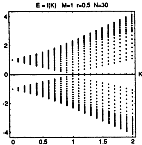
Figure 2. Energy levels versus hopping parameter K for Wilson fermions on a 30 site lattice.
