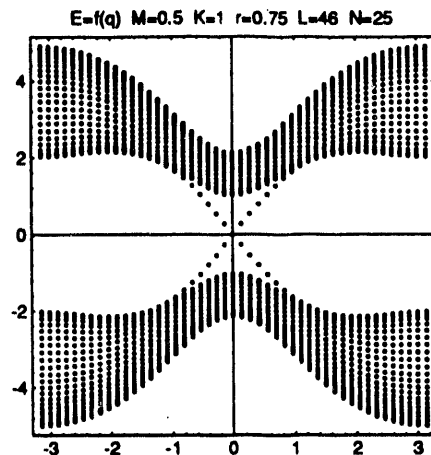
Figure 3. The energy spectrum as a function of the physical momentum on a lattice with 46 space sites and 25 sites in the extra dimension. Note the crossing surface modes at low energy.
