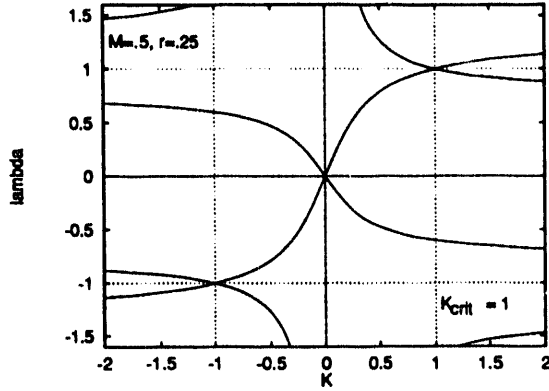
Figure 5. The translation eigenvalues at zero energy as a function of the hopping parameter. Note the crossing at the critical hopping K = 1 . Here r = .25 and M = .5 .
