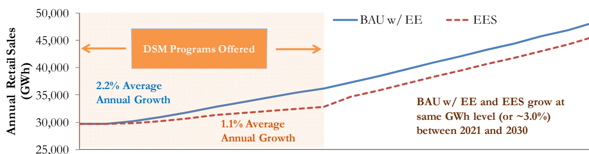
Figure 2. Effect of energy efficiency portfolios on Arizona utility load forecast
