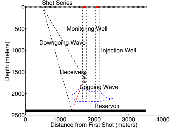
Figure 1: The schematic configuration of the walkaway VSP surveys at SACROC.
