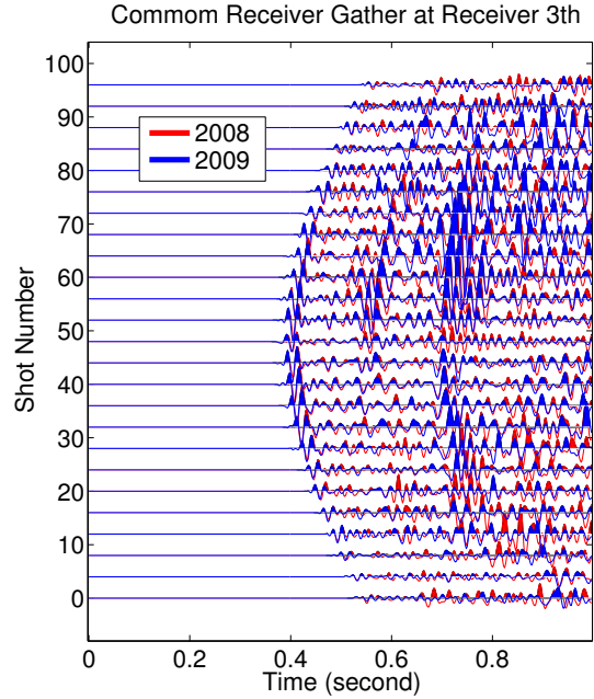
Figure 2: Upgoing waveforms of the baseline walkaway VSP survey in 2008 (in red) and those of the repeat survey in 2009 (in blue) recorded by the third borehole receiver. The data were acquired at an EOR field at SACROC.
