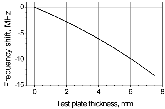
Fig. 3. Computed the cavity frequency shift vs. the test plate thickness.
