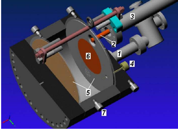
Fig. 1. The model of the cavity for cooling of muons. 1- vacuum port, 2- antenna, 3- RF coax feeder, 4- probe, 5- test plate holder, 6- test plate to study materials at high gradients of RF field, 7- roller.
