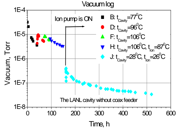
Fig. 2. Vacuum log of the 805 MHz pillbox RF cavity.
