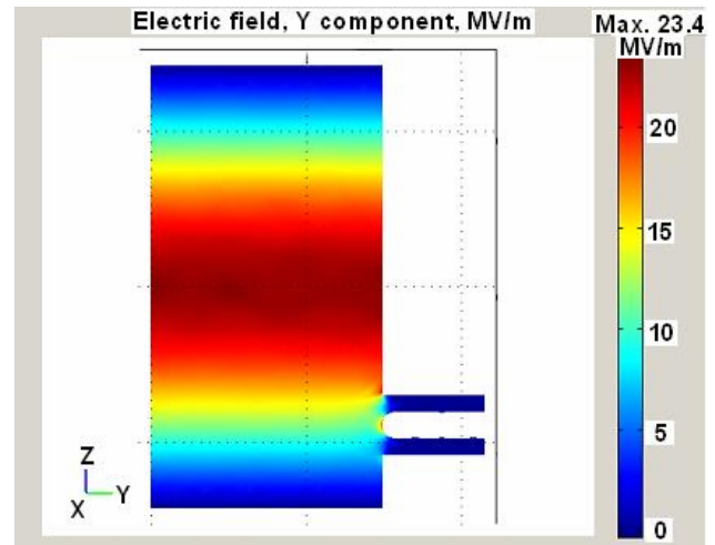
Fig. 5. Computed the RF electric field distribution in the pillbox cavity at 1 MW RF power and critical coupling of the cavity.
