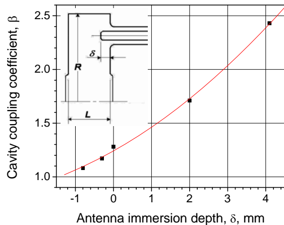
Fig. 4. Measured the cavity coupling coefficient vs. the antenna immersion depth.
