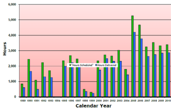
Figure 3: Operating hours for the Lujan Center illustrate recent stability at over 3,000 scheduled hours per year.
